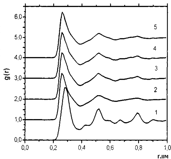
Fig. 16. Radial distribution function g(r) for Ta-Fe melt at 3400 K temperature, obtained in MD model at 15.4 \text{ g/cm}^3 liquid Ta density. 1. No electric field, no hydrogen, 2. Electric field 85 [V/m], no hydrogen, 3. Hydrogen, no electric field, 4. Electric field 85 [V/m], Hydrogen, 5. Electric field 1020 [V/m], Hydrogen.
