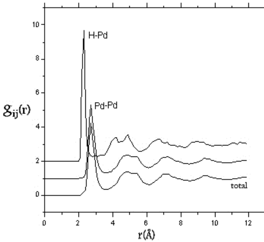
Fig. 7. Partial RDF in an amorphous Pd-H - system.
