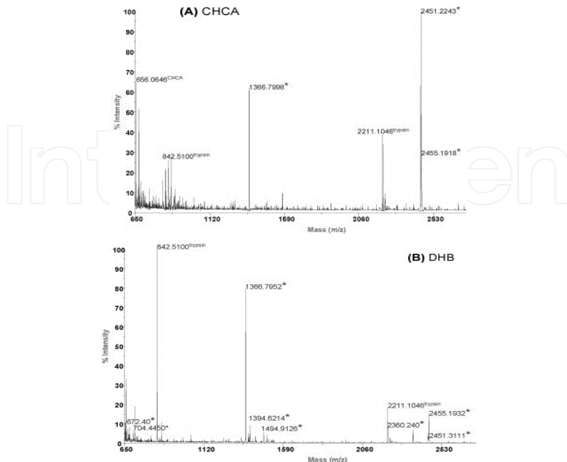
Fig. 12. Comparison of \alpha -cyano-4-hydroxycinnamic acid (CHCA) and 2,5-dihydroxybenzoic acid (DHB) as matrices in MALDI-TOF MS of a silver stained protein.
