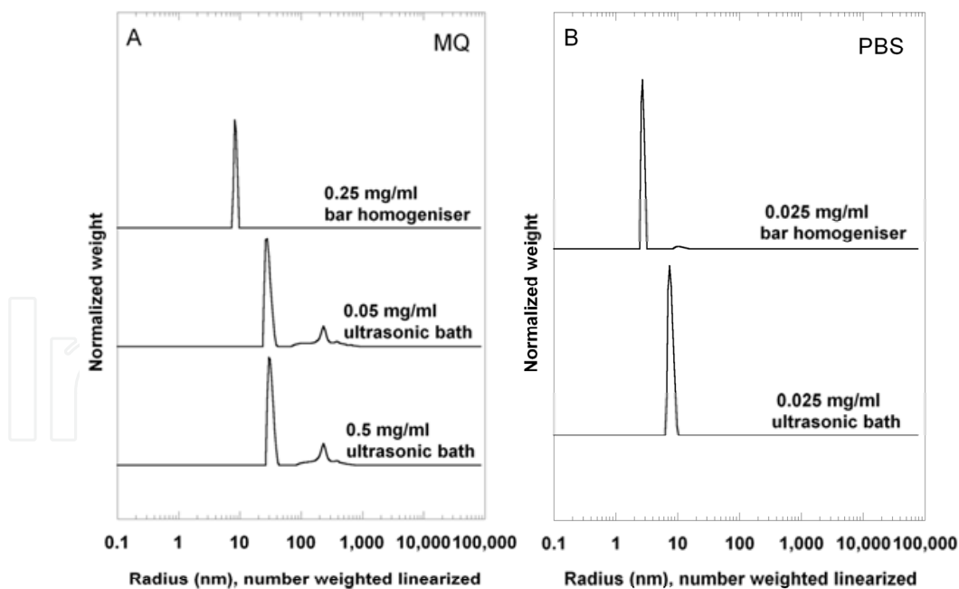
Fig. 3. DLS measurements of ZnO (Aluminium 6% doped) nanoparticles.
