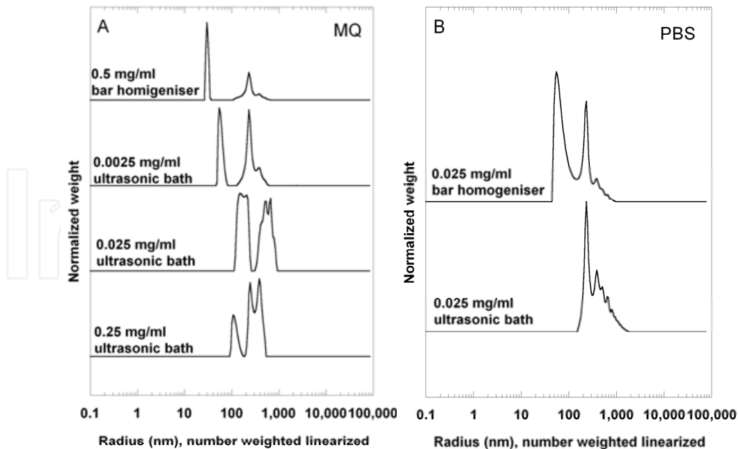
Fig. 2. DLS measurements of \text{Al}_2\text{O}_3 nanoparticles.
