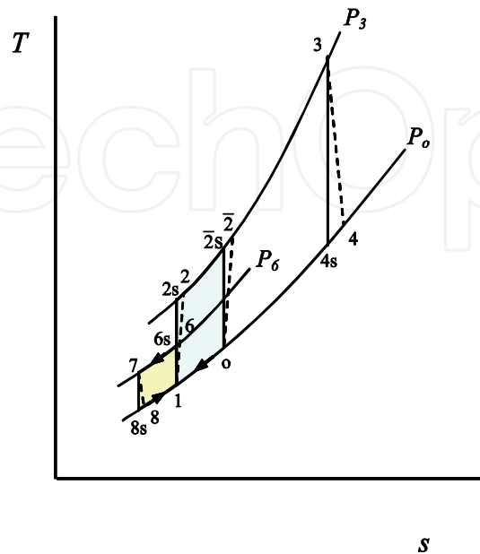
Fig. 2. T - s diagram for the proposed cycle
