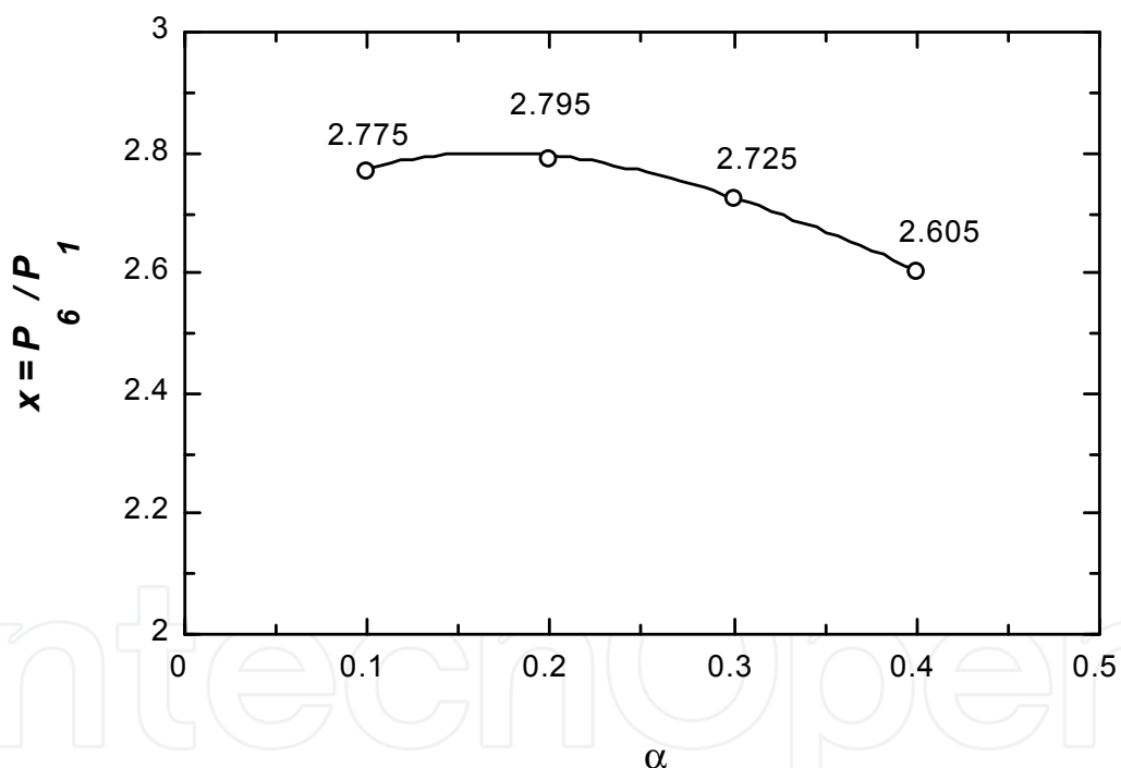
Fig. 3. Solution of Eq. 39, TEC = 0 gives the conditions for constant thermal efficiency
