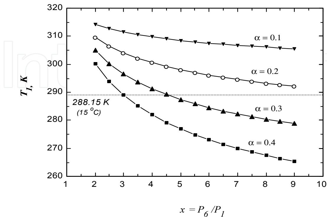
Fig. 4. Effect of extraction pressure x and mass ratio \alpha on the gas turbine intake air temperature.
