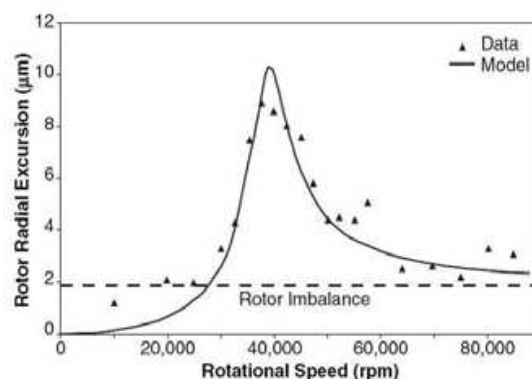
Fig. 11. Behaviour of an air micro bearing [Epstein 1997]
