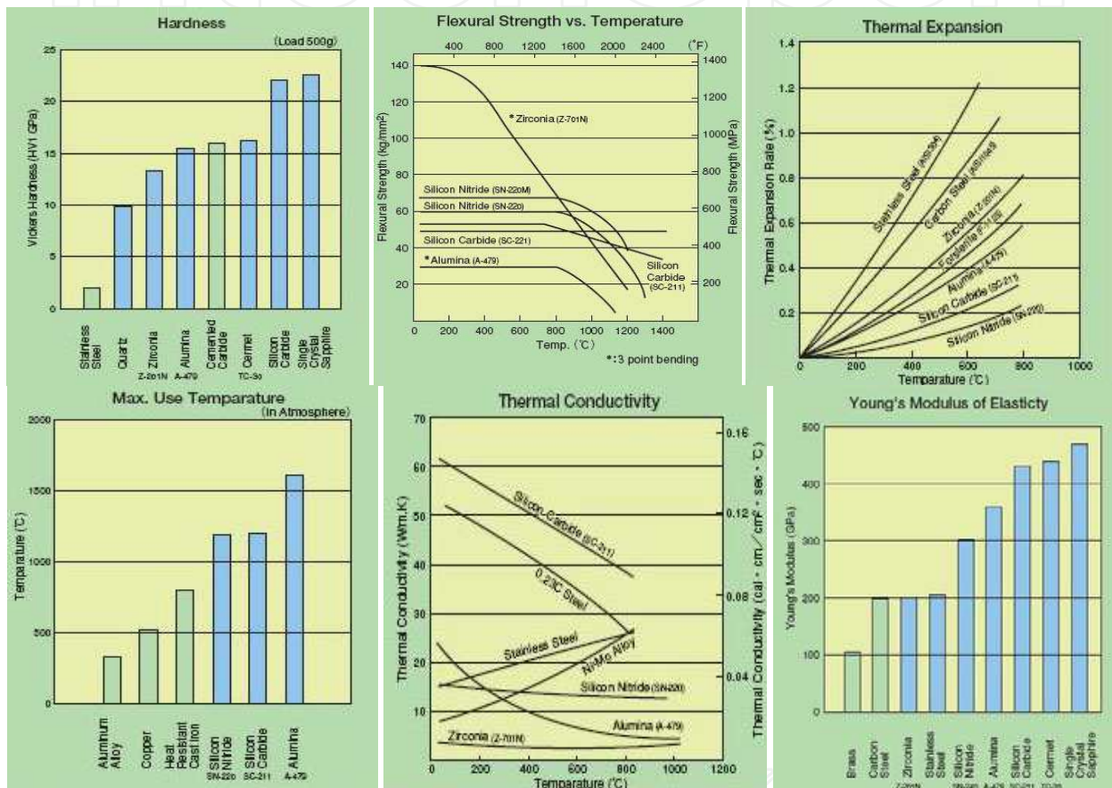
Fig. 13. Materials characteristics
