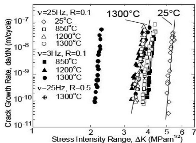
Fig. 19. Si 3 N 4 Stress intensity range
