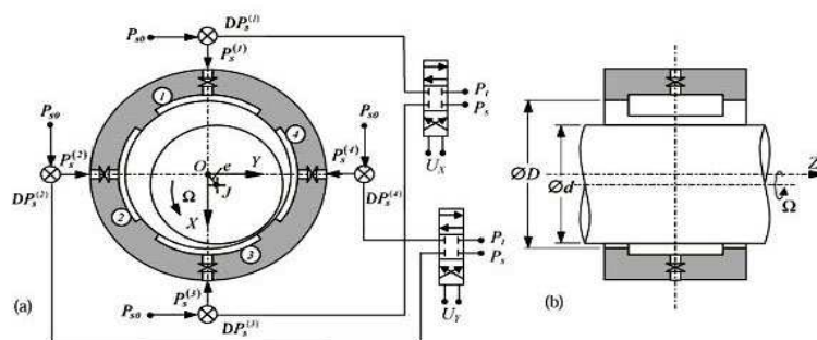
Fig. 9. Hybrid configuration
