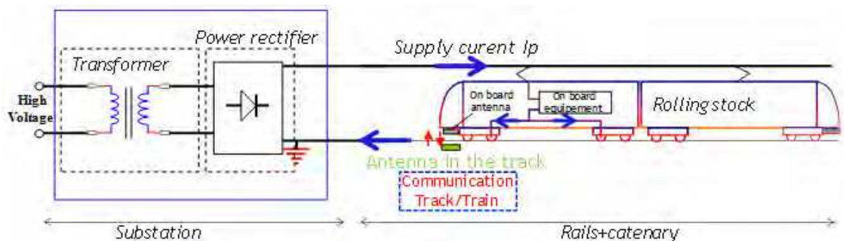
Fig. 3. Simplified diagram of railway infrastructure
