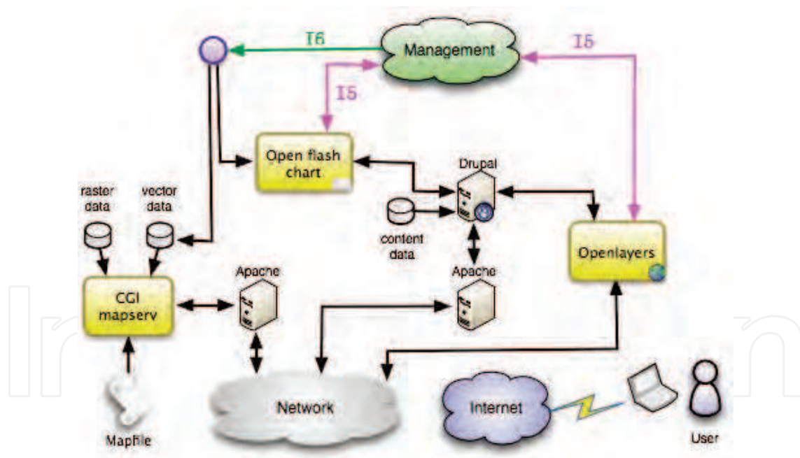
Fig. 24. Visualization Module Architecture.
