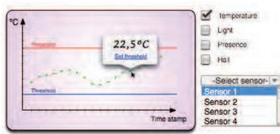
Fig. 26. User interaction over a graphics view.
