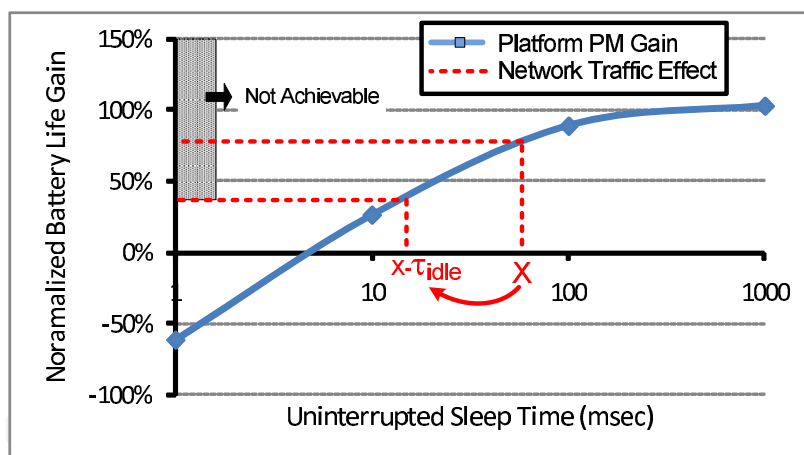
Fig. 4. Traffic Effect on PM Energy Gain
