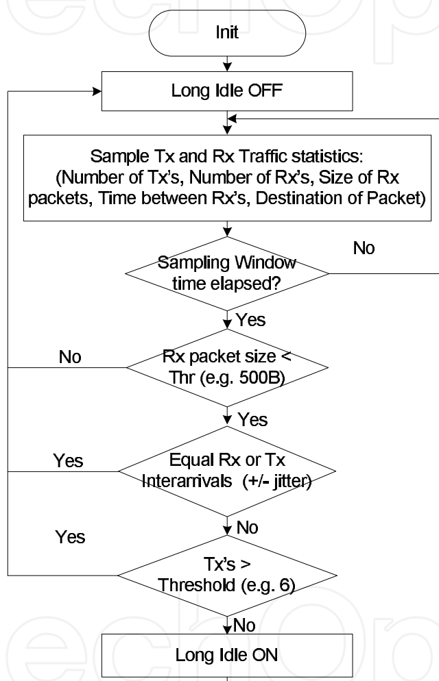
Fig. 8. Long Idle Sampling State Machine
