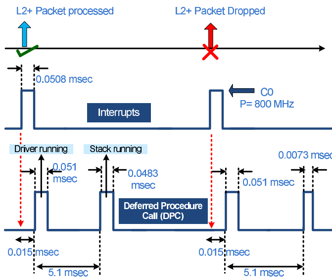
(b) Cost for L2+ Packets
