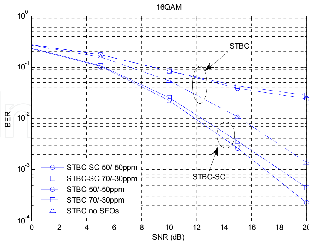
Fig. 13. BER of STBC and STBC-SC (16QAM)
