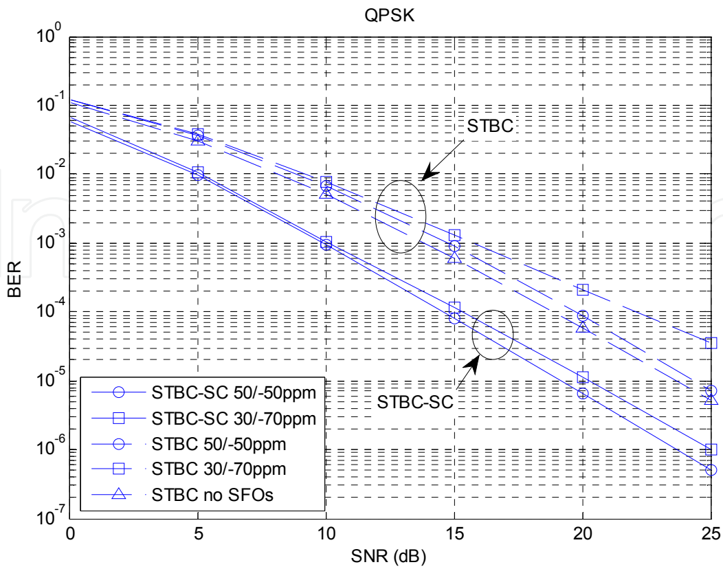
Fig. 12. BER of STBC and STBC-SC (QPSK)
