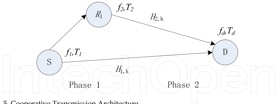
Fig. 5. Cooperative Transmission Architecture
