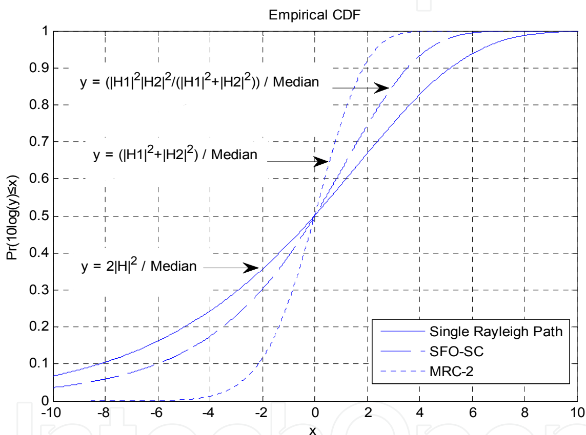
Fig. 2. Diversity gain from Symmetric Combination
