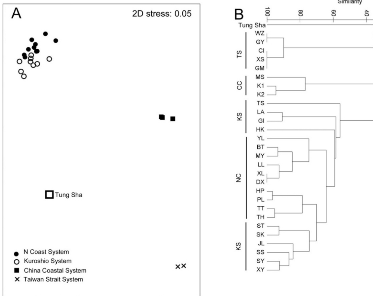
Fig. 2. A. Non-metric nMDS plots on the species composition in all sites from the N Coast Ecosystem, Taiwan Strait Ecosystem and the China Coastal Ecosystem. B. Cluster plots on the species composition on all sites from the N Coast Ecosystem (NC), Kuroshio Ecosystem (KS), Taiwan Strait Ecosystem (TS) and the China Coastal Ecosystem (CC). Tung Sha was not grouped in the ecosystem because it is located in the South China Sea. The Taiwan Strait Ecosystem and the China Coastal Ecosystem overlap in the ordination plot.
