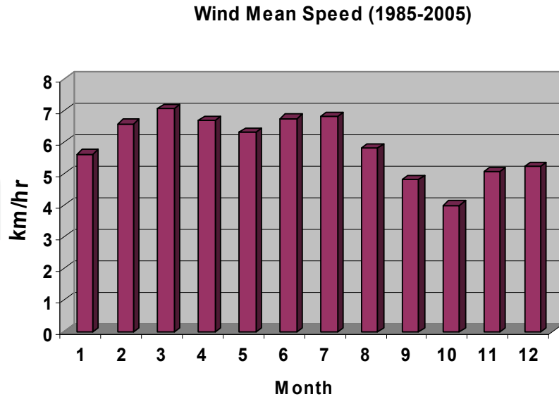
Fig. 23. Average monthly wind speed
