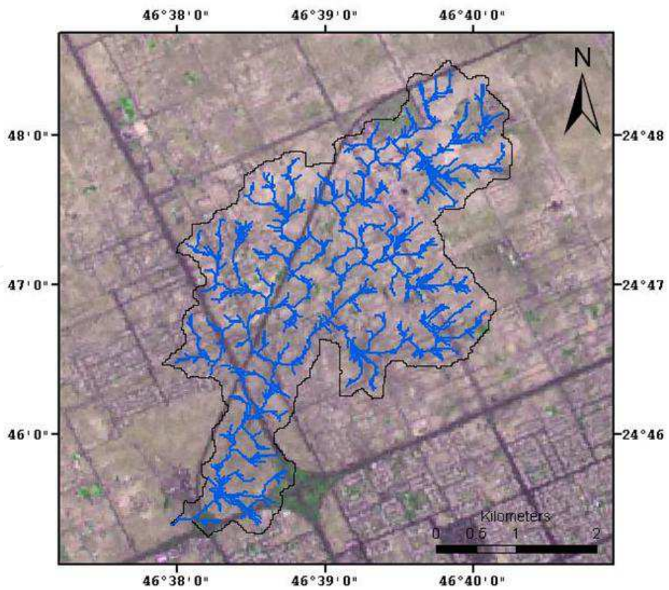
Fig. 17. Detailed drainage system of the site and its surroundings.
