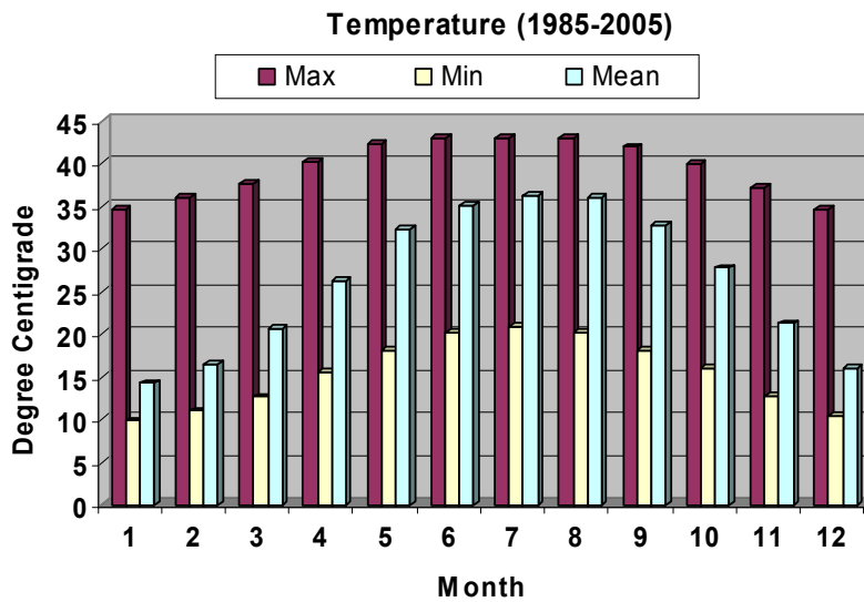
Fig. 20. Minimum, maximum, and average monthly temperature.
