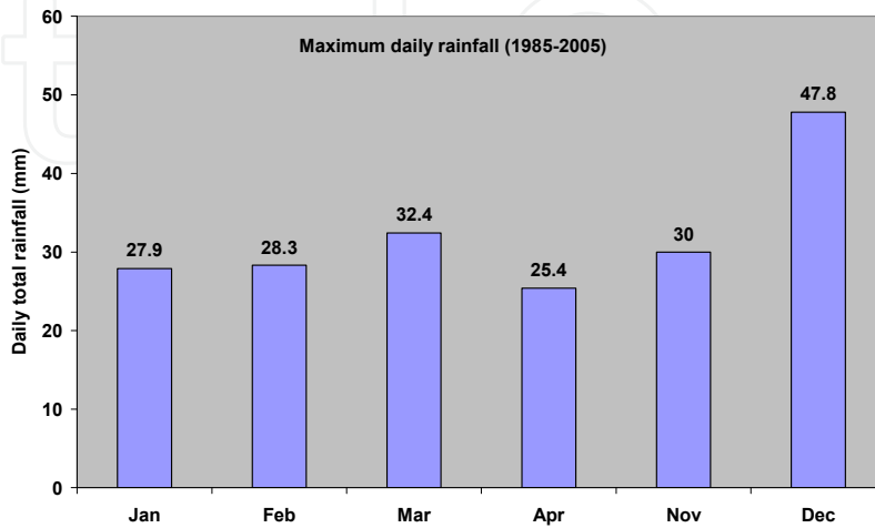
Fig. 19. Maximum daily total rainfall
