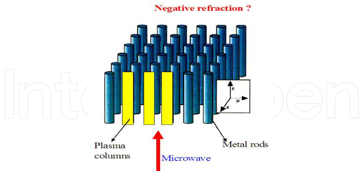
Fig. 3. Hybrid plasma photonic crystal
