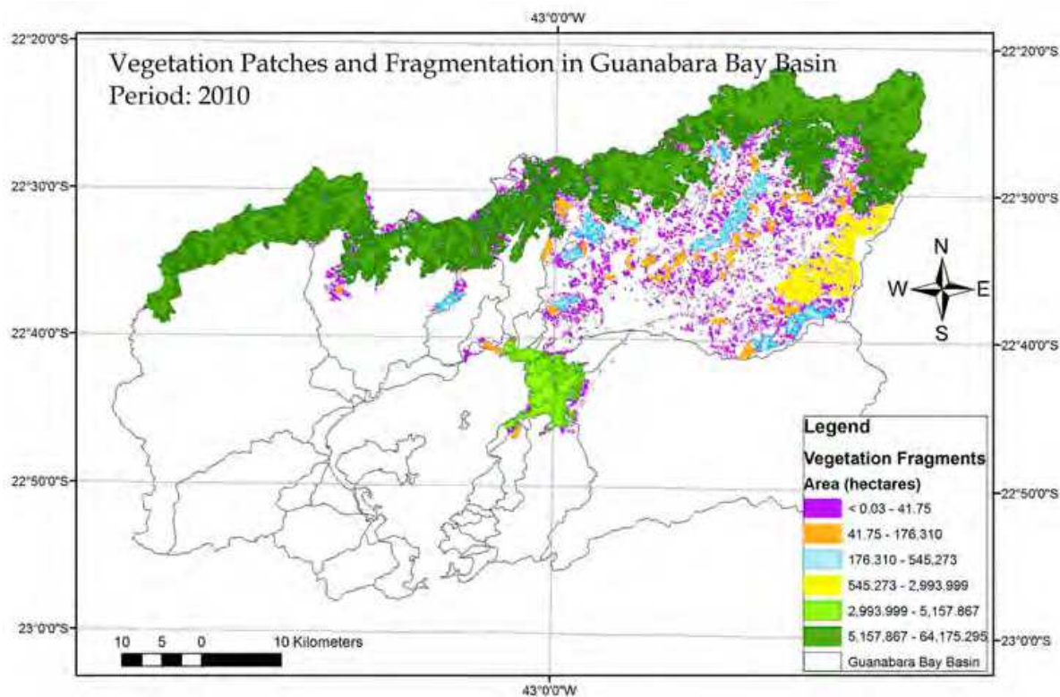
Fig. 14. Vegetation Fragmentation in Guanabara Bay Basin (2010)
