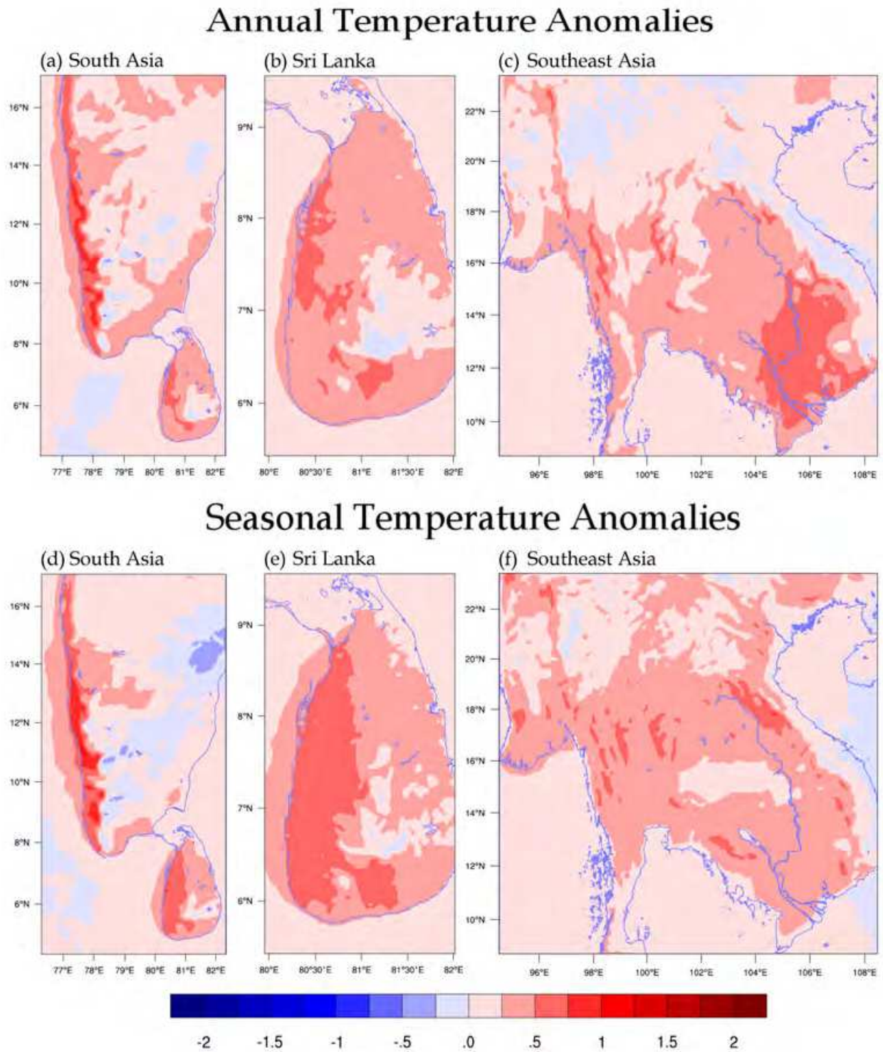
Fig. 1. The annual and the seasonal (June, July and August) temperature anomalies (i.e. deforest -forest) for South Asia (a,d), Sri Lanka (b,e) and Southeast Asia (c,f) for 1988. Temperature is the surface air temperature 2m above the surface and is expressed in Kelvins (K) with a contour interval of 0.25 K.
