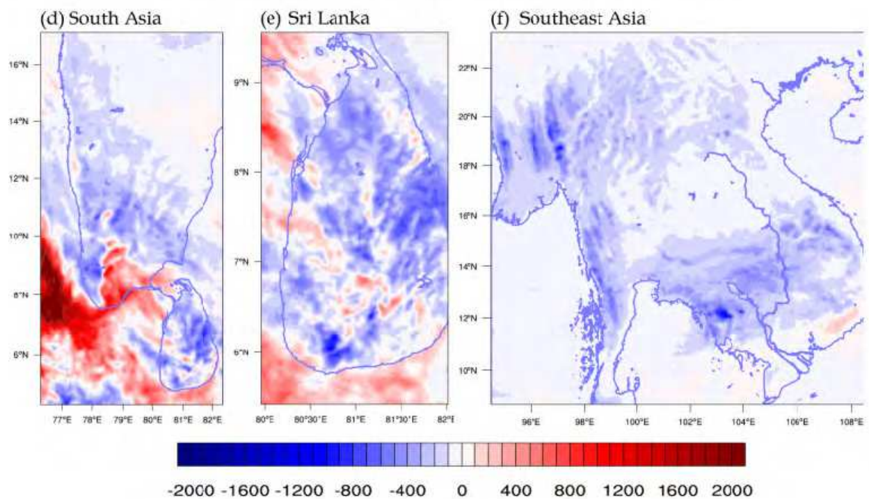
Fig. 3. The total annual and the seasonal (June, July and August) precipitation anomalies (i.e. deforest -forest) for South Asia (a,d), Sri Lanka (b,e) and Southeast Asia (c,f) for 1988. Precipitation is in millimeters (mm) with a contour interval of 100 mm.
