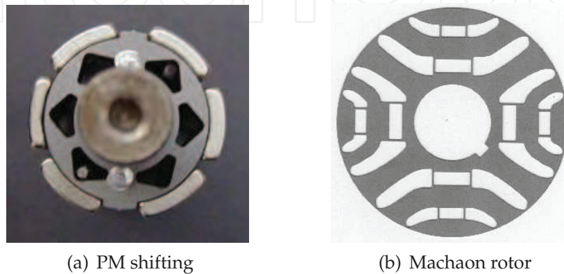
Fig. 18. Photos of proper solutions to optimize the torque behavior.
