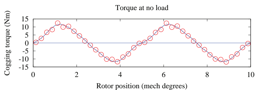
Fig. 12. Cogging torque versus rotor position.
