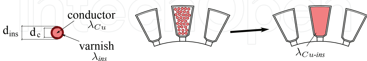
Fig. 29. Thermal equivalent model of the slot
