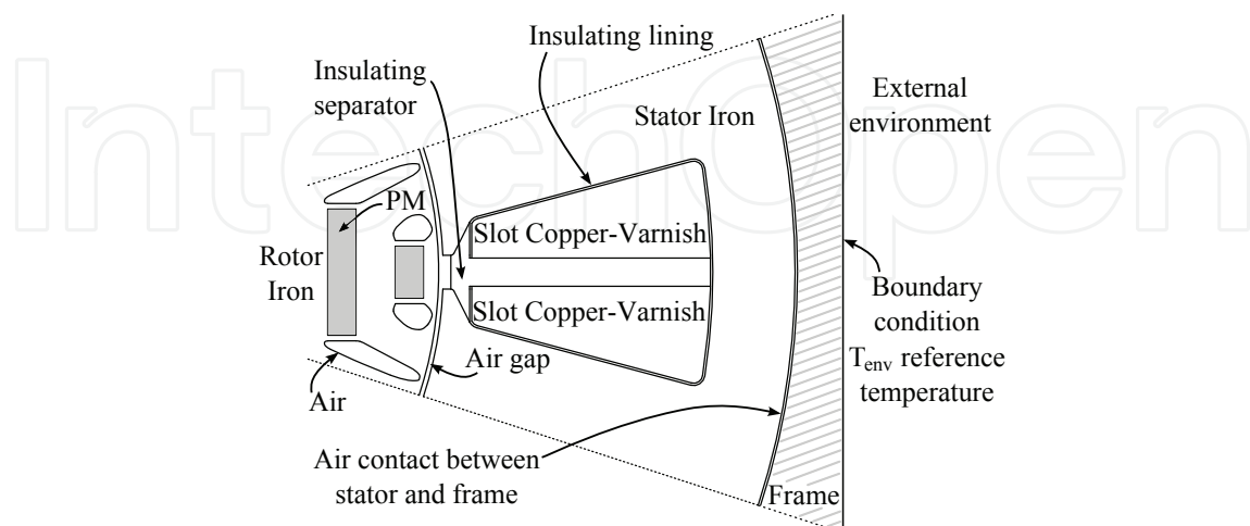
Fig. 28. Detail of machine geometry and material properties adopted in the FE analysis.
