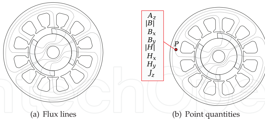
Fig. 7. Flux lines and magnetic quantities detected in the point P of the solved structure.
