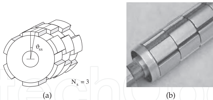
Fig. 13. Stepped rotor skewing with three modules
