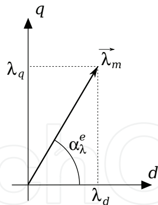
Fig. 9. Flux linkage space vector and its components.
