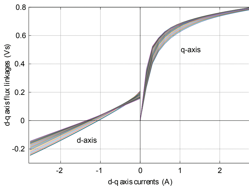
Fig. 15. d - q axis flux linkages versus currents.
