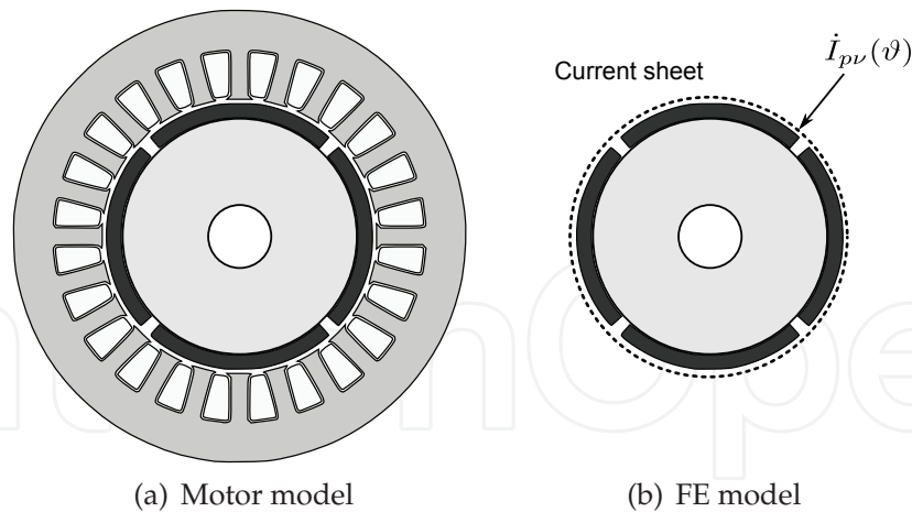
Fig. 25. Model used for FE computations.
