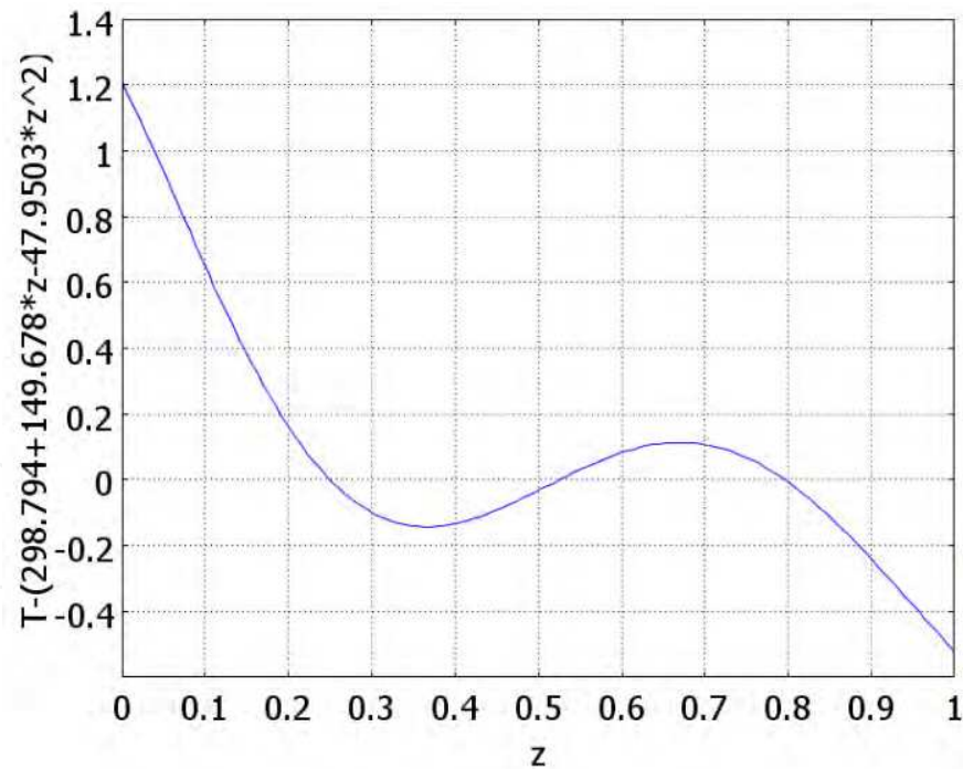
Fig. 30. Variant 2, start simplex B - Disparity between the expected and the obtained temperature distribution
