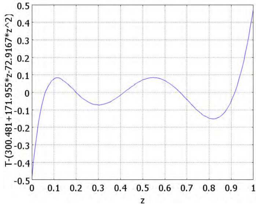
Fig. 20. Variant 2, start simplex C - Disparity between the expected and the obtained temperature distribution
