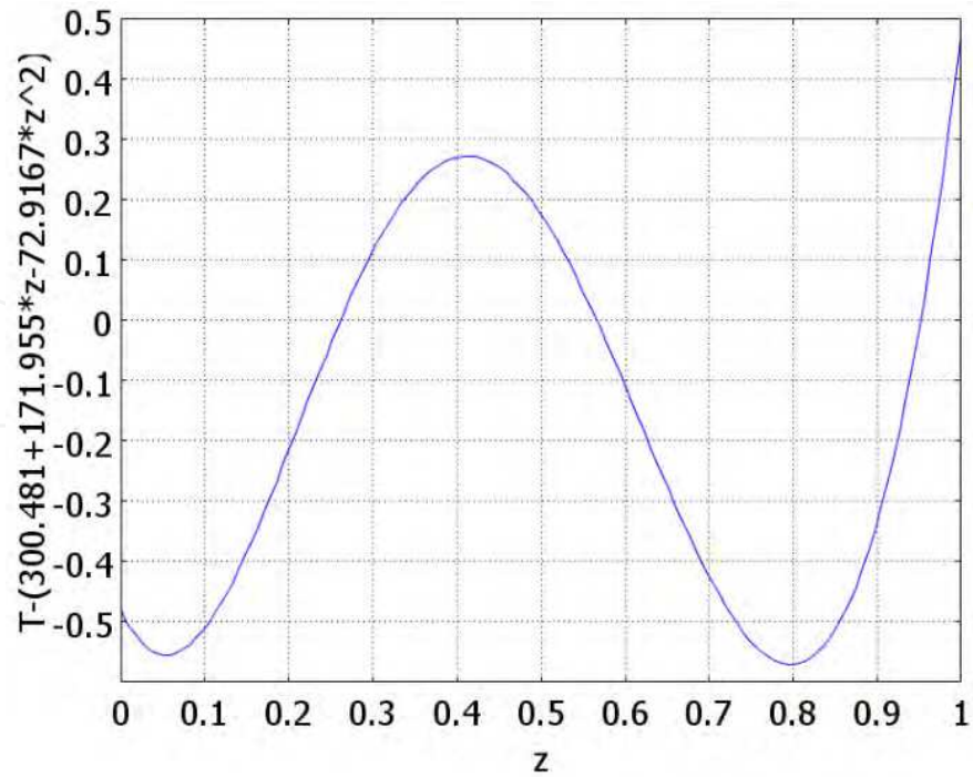
Fig. 18. Variant 2, start simplex B - Disparity between the expected and the obtained temperature distribution
