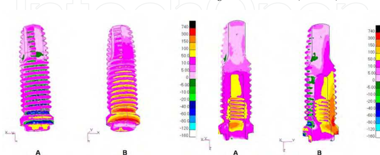
Fig. 16. Perspective and internal view of the implant. Maximum principal stresses in model with a load of 45° on the vestibular cusp.
