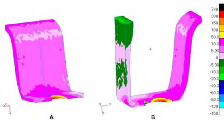
Fig. 30. Internal view of the cortical bone. Maximum principal stresses in model with a load of 45° on the mesial marginal ridge. In A, mesio-distal section; in B, vestibulo-lingual section.
