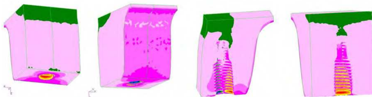
Fig. 15. Perspective and internal view of the cancellous bone. Maximum principal stresses in model with a load of 45^\circ on the vestibular cusp.
