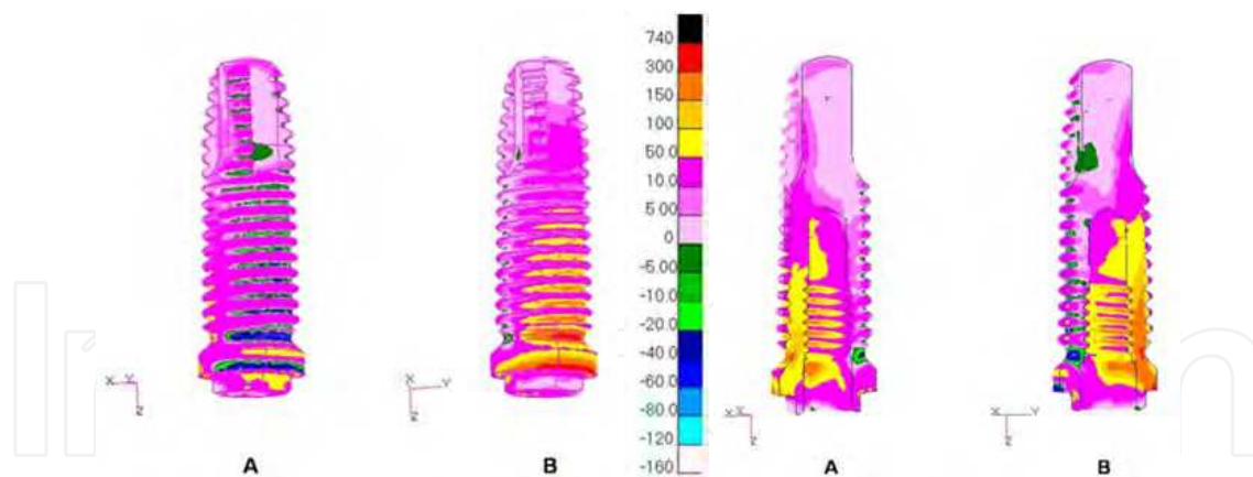
Fig. 32. Perspective view of the implant. Maximum principal stresses in model with a load of 45° on the mesial marginal ridge.
