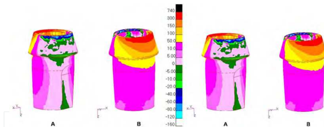
Fig. 34. Perspective and internal view of the abutment. Maximum principal stresses in model with a load of 45° on the mesial marginal ridge.
