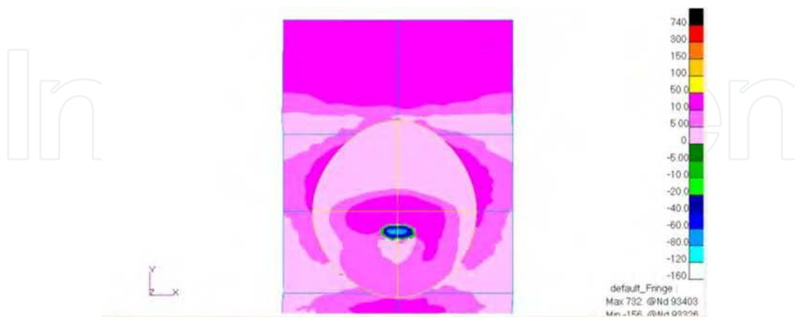
Fig. 12. Occlusal view. Maximum principal stresses in model with a load of 45° on the vestibular cusp.
