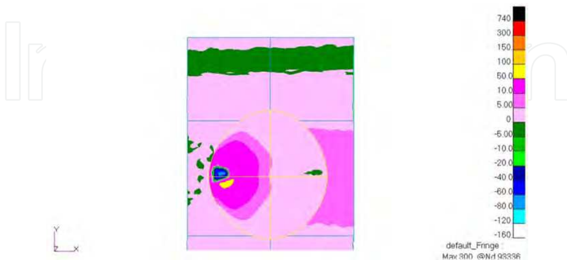
Fig. 20. Occlusal view. Maximum principal stresses in model with a load of 0° on the mesial marginal ridge.
