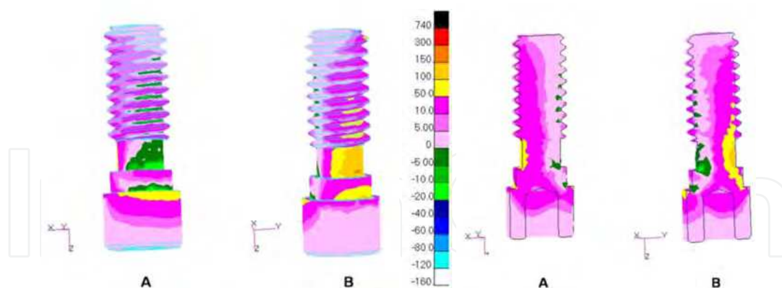
Fig. 33. Perspective view of the screw. Maximum principal stresses in model with a load of 45° on the mesial marginal ridge.
