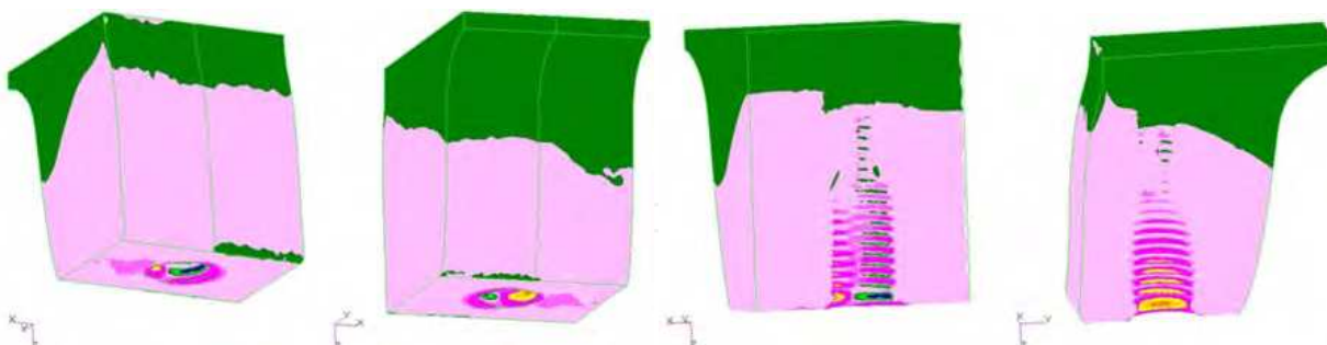
Fig. 23. Perspective and internal view of the cancelous bone. Maximum principal stresses in model with a load of 0° on the mesial marginal ridge.
