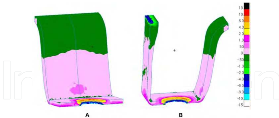
Fig. 6. Internal view of the cortical bone. Maximum principal stresses in model under longitudinal load. In A, mesio-distal section; in B, vestibulo-palatine section.
