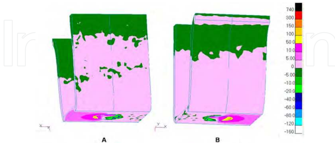
Fig. 21. View of the cortical bone. Maximum principal stresses in model with a load of 0^\circ on the mesial marginal ridge. In A, disto-vestibular view; in B, mesio-palatine view.
