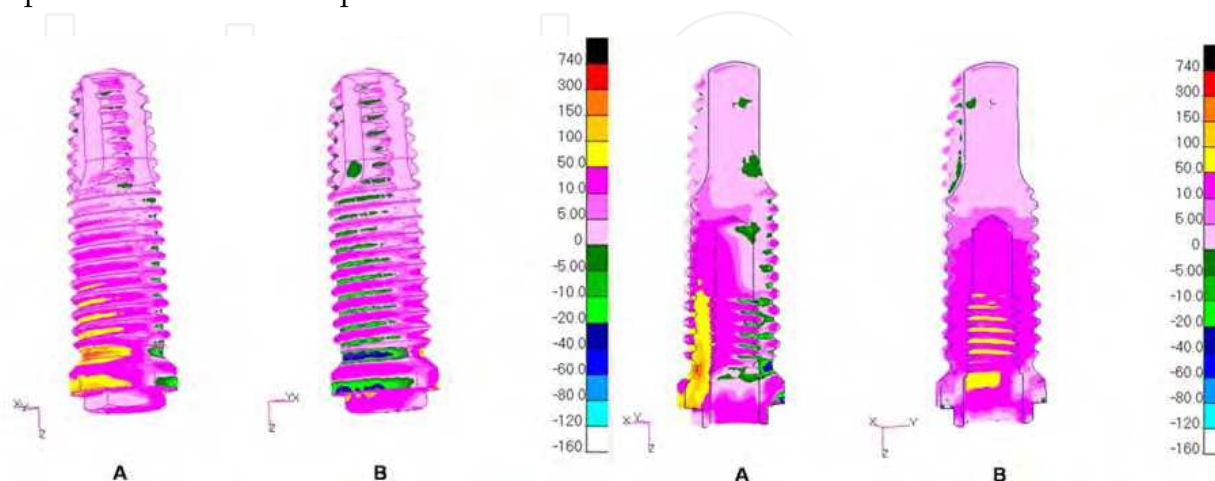
Fig. 24. Perspective and internal view of the implant. Maximum principal stresses in model with a load of 0° on the mesial marginal ridge.
