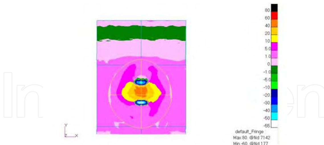
Fig. 4. Occlusal view. Maximum principal stresses in model under longitudinal load.
