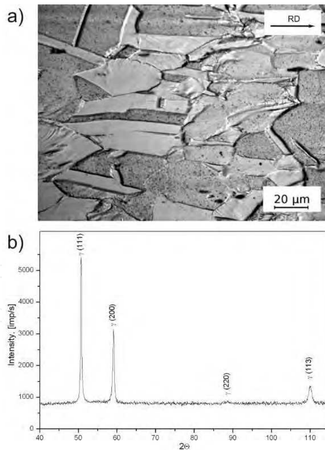
Fig. 3. Austenitic structure with annealing twins of 26Mn-3Si-3Al-Nb steel after the thermo-mechanical rolling and immersion in 1N H 2 SO 4 (a) and X-ray diffraction pattern (b).
