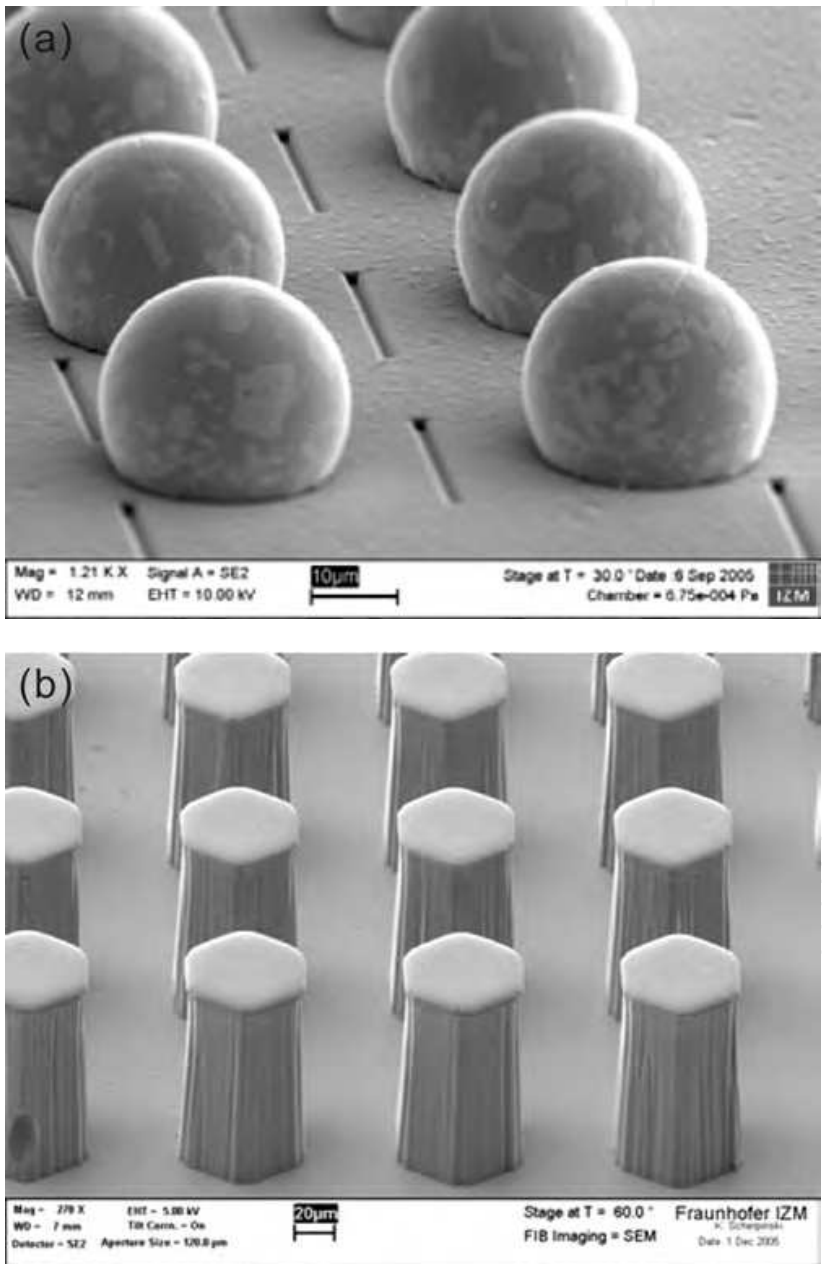
Fig. 1. Micro bump and pillar bump structures for highly reliable chip-to-substrate interconnects: (a) SnAg microbump (20 µm diameter), and (b) Cu pillarbump (height: 80 µm) [11]
