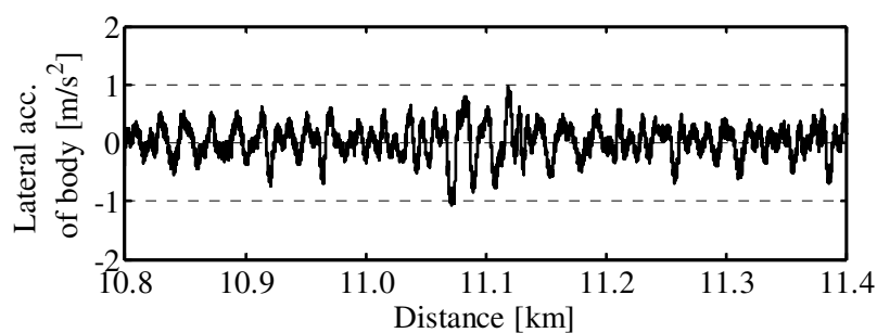
(a) Lateral acceleration of car body
