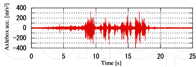
(a) Vertical acceleration of axle-box
