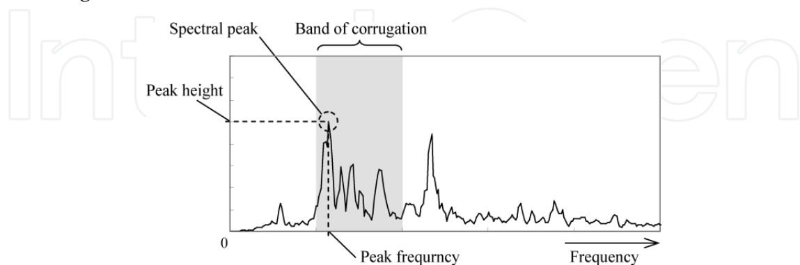
Fig. 11. Detection of corrugation from cabin noise
