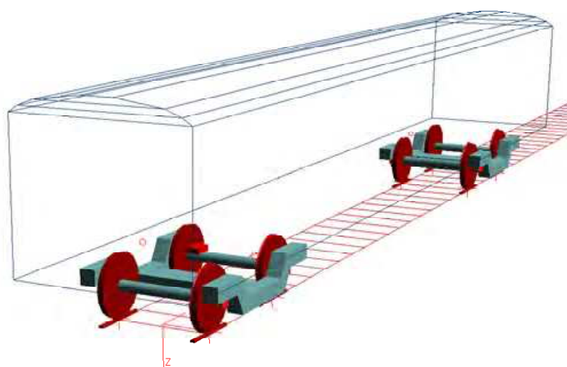
Fig. 9. Full vehicle model
