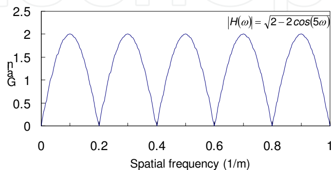
Fig. 27. Frequency response of difference filter
