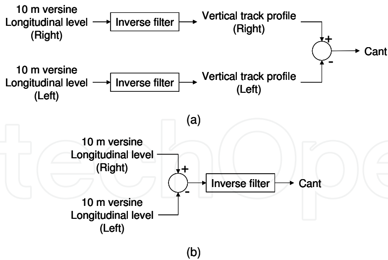
Fig. 30. Calculation flow for cant
