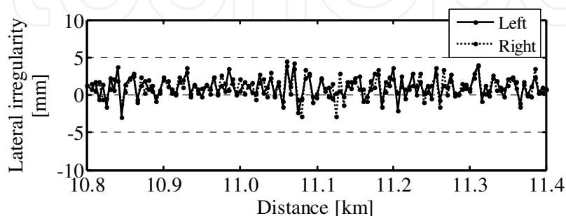
(c) Lateral irregularity of track
