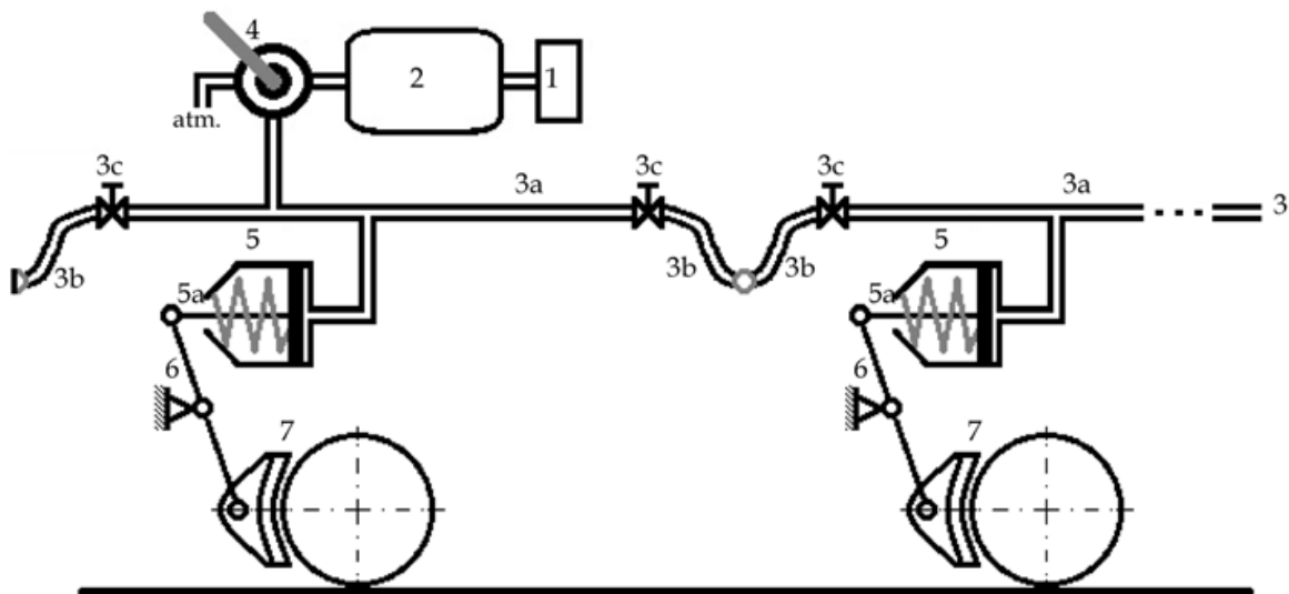
Fig. 1. Schematic of straight compressed air brake system:
