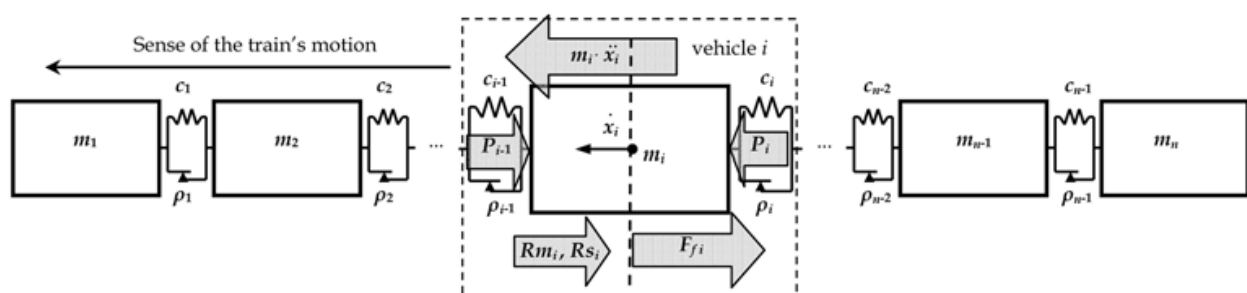
Fig. 14. Mechanical model of the train
