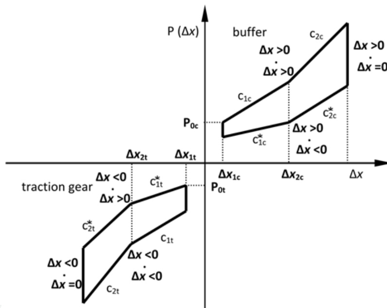
Fig. 15. General characteristics of shock (index c) and traction gear (index t) devices.
