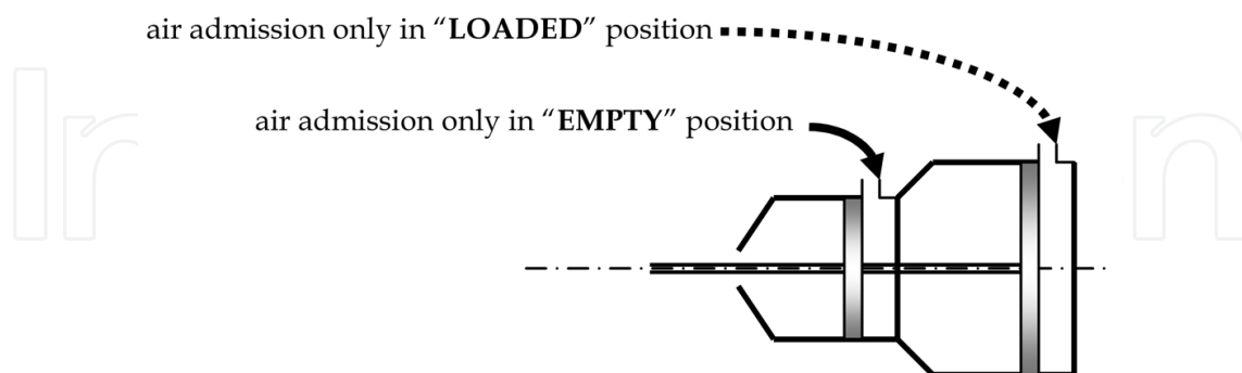
Fig. 12. Double brake cylinder.
