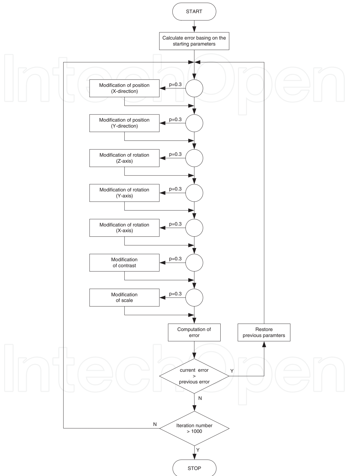
Fig. 13. Evolutionary optimization
