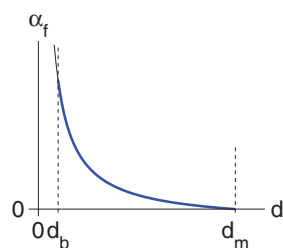
Fig. 11. The obstacle-avoidance gain \alpha_f versus the distance to the obstacle
