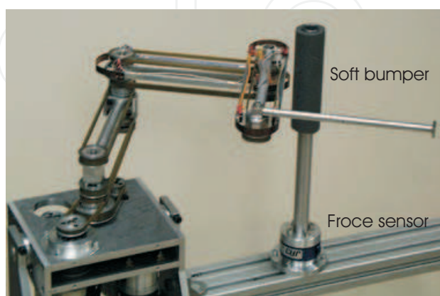
Fig. 13. Experimental manipulator with external force sensor
