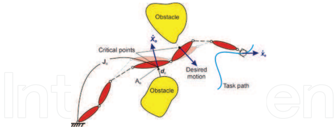
Fig. 1. Manipulator motion in presence of some obstacles
