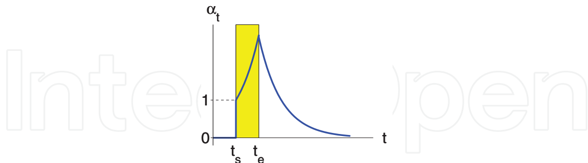
Fig. 9. The obstacle-avoidance gain \alpha_t versus the duration of the contact
