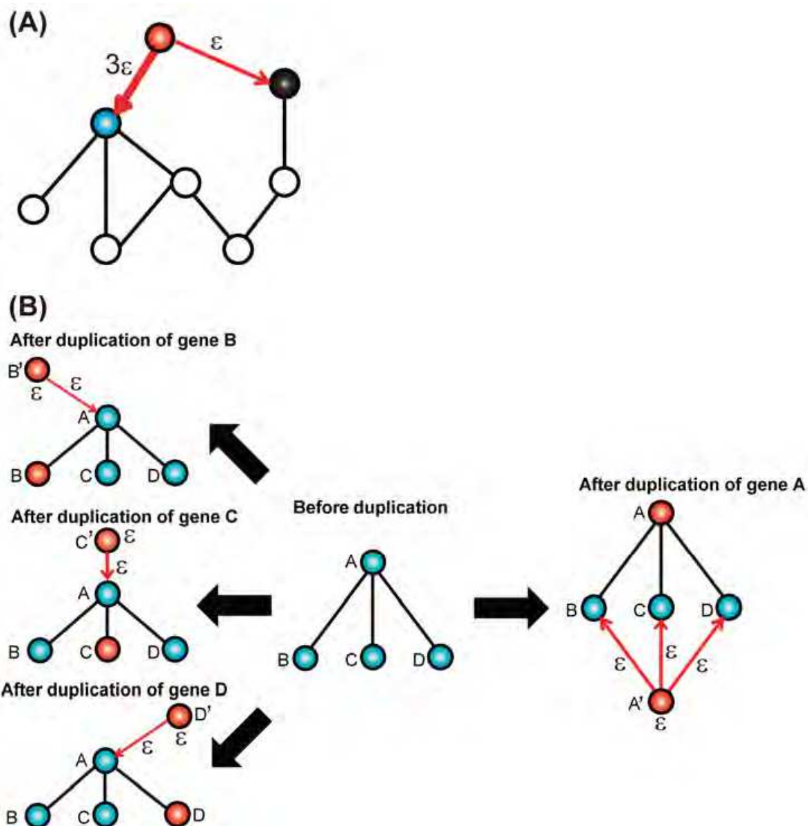
Fig. 2. Network growth by preferential attachment (A) Preferential attachment. A red node is added to the network. The probability that a new link is attached between red and blue nodes ( 3\epsilon ) is three times higher than that between red and black nodes ( \epsilon ). (B) Network growth with gene duplication. Red nodes represent duplicated nodes. Gene duplication occurs with an equal probability ( \epsilon ) for all nodes. When node A is duplicated, degrees of nodes B, C, and D increase by one (right), whereas when either node B, C, or D is duplicated, degree of node A increases by one (left).
