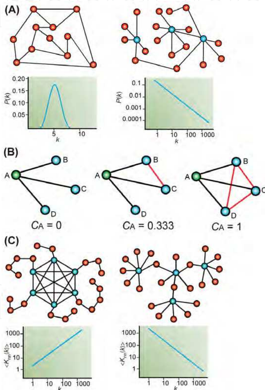
Fig. 1. Measures of a network structure
