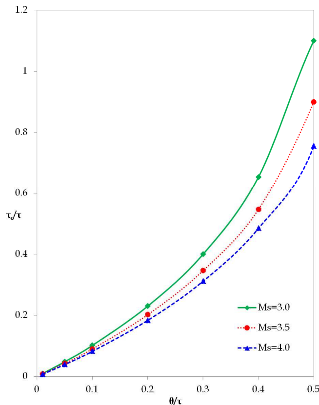
Fig. 15. \tau_c guidelines for a FODUP
