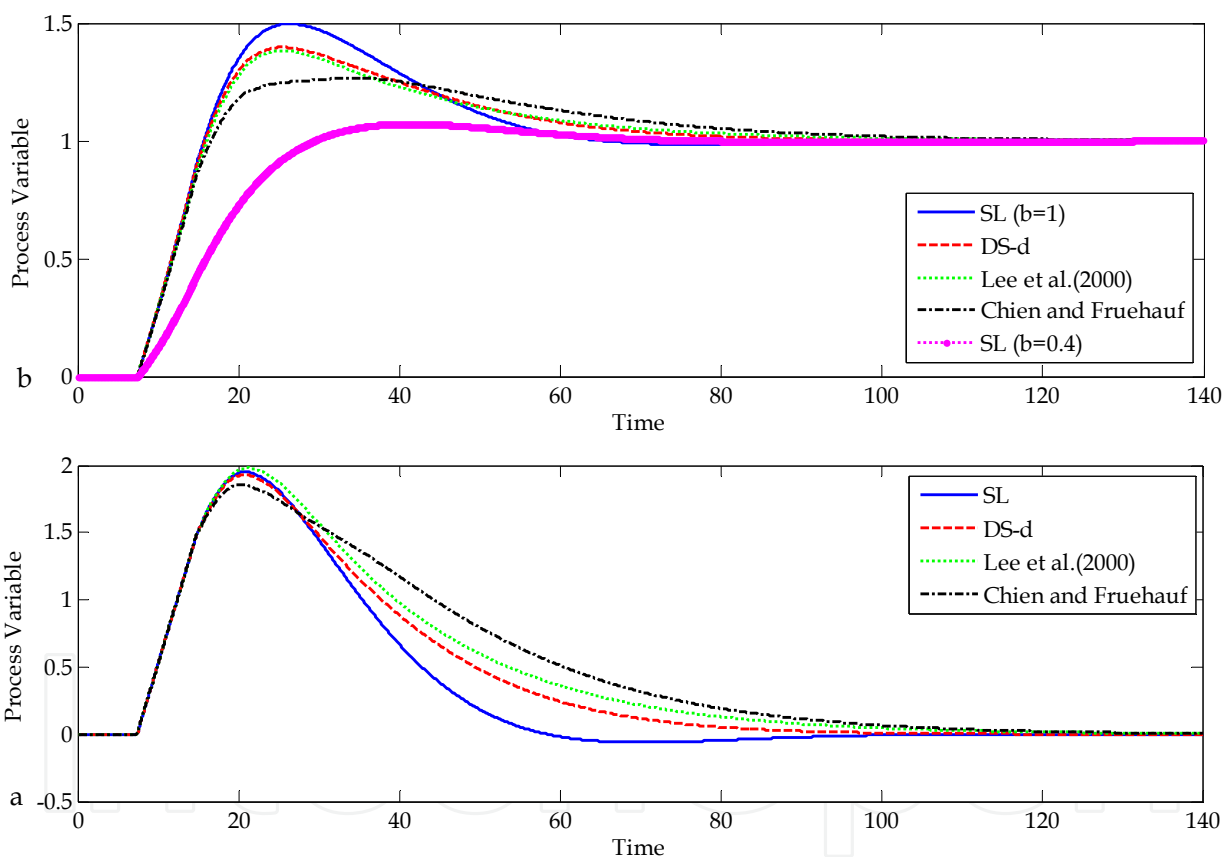
Fig. 3. Responses of the nominal system in Example 2.
