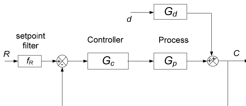
(b) Classical feedback control structure
