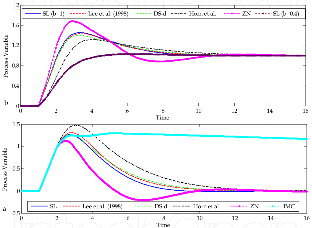
Fig. 2. Responses of the nominal system in Example 1.
