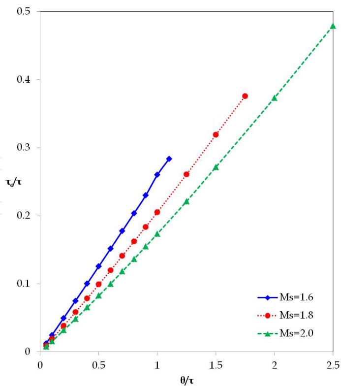
Fig. 14. \tau_c guidelines for a FODIP
