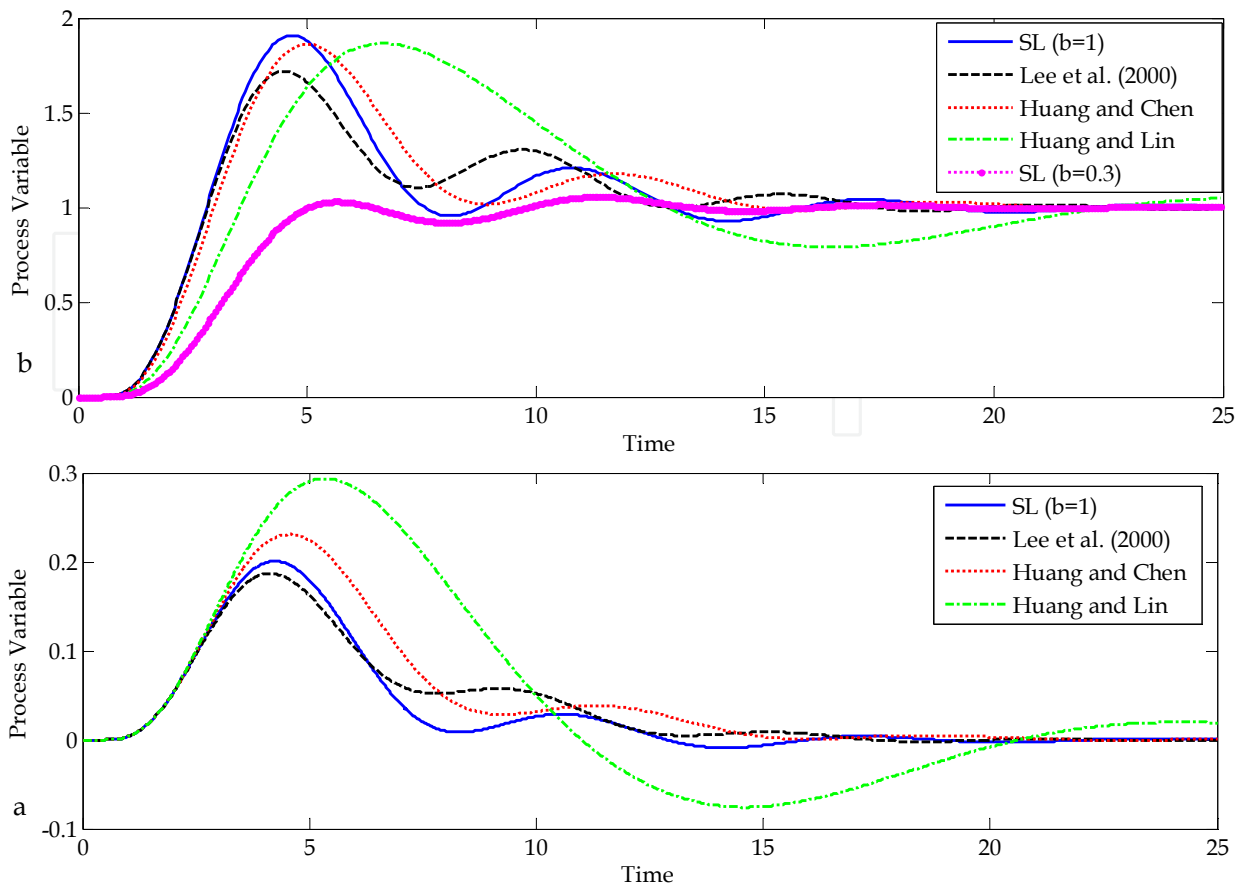
Fig. 7. Responses of the nominal system in Example 6.
