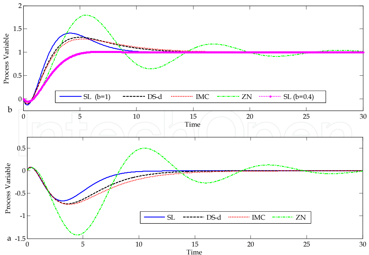
Fig. 5. Responses of the nominal system in Example 4.
