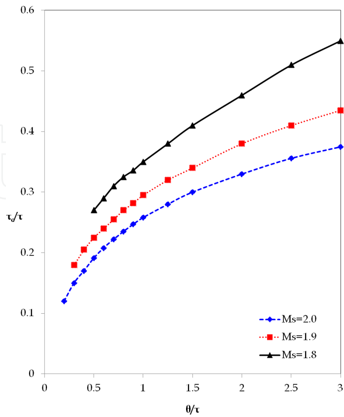
Fig. 13. \tau_c guidelines for a SOPDT
