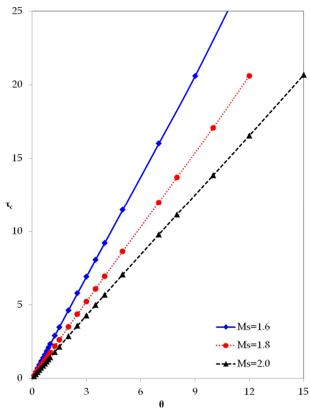
Fig. 11. \tau_c guidelines for a FOPDT
