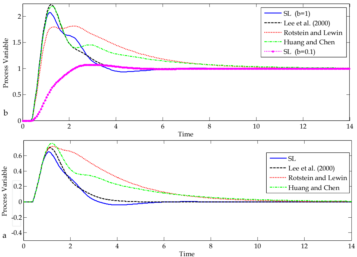
Fig. 6. Responses of the nominal system in Example 5.
