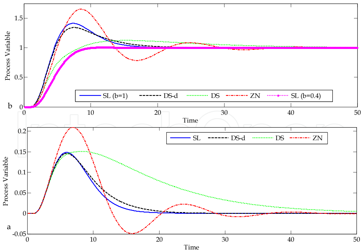
Fig. 4. Responses of the nominal system in Example 3.
