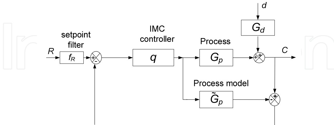
(a) The IMC structure
