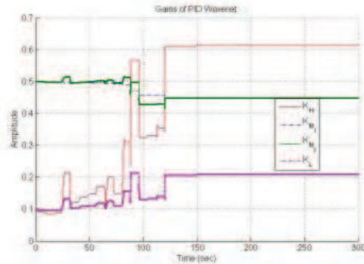
Fig. 27. Results of the wavenet PID gains
