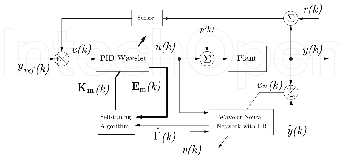
Fig. 23. Close loop block diagram of a SISO system with wavenet PID
