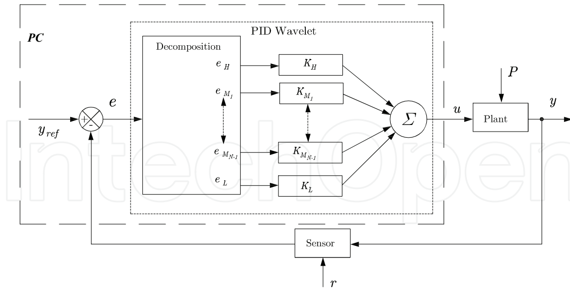
Fig. 4. Close loop block diagram of a SISO system with the MRPID controller.
