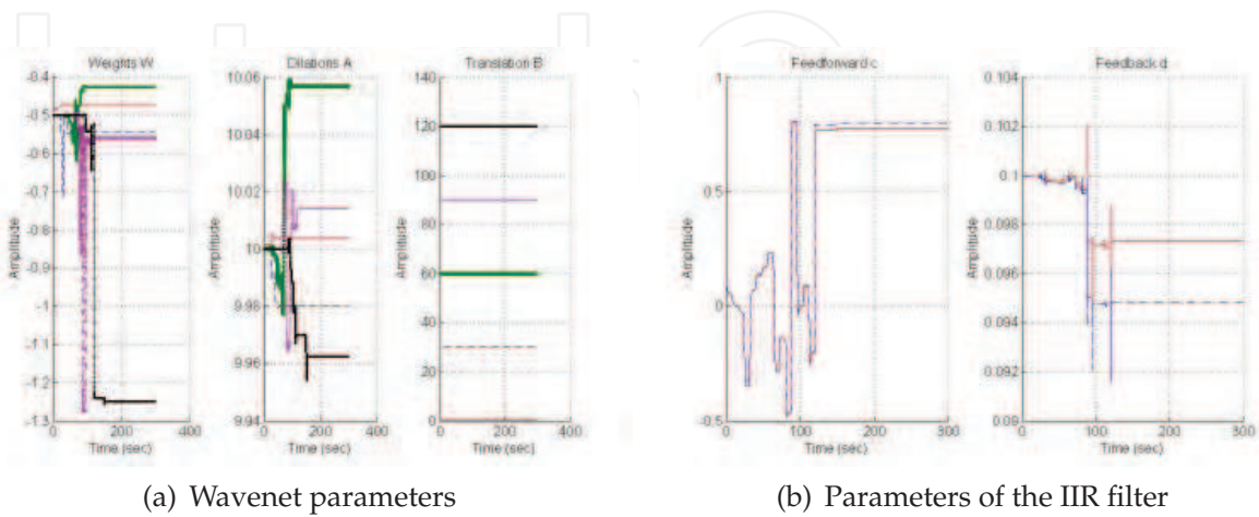
Fig. 26. Results of parameters of the wavelet neural network
