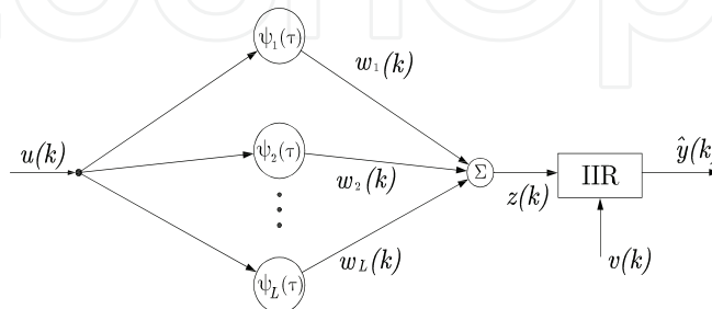
Fig. 22. Structure of wavelet network with IIR filter
