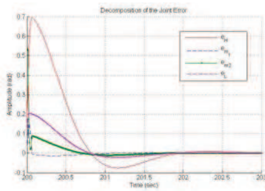
Fig. 25. Decomposition of the error signal
