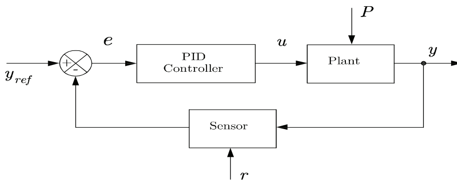
Fig. 2. Scheme of a SISO system with a PID controller.
