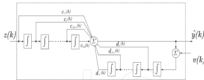
Fig. 21. Scheme block diagram of IIR filter model
