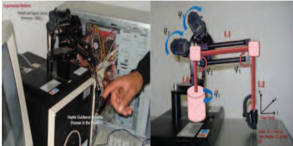
Fig. 14. Haptic interface PHANToM Premium 1.0.
