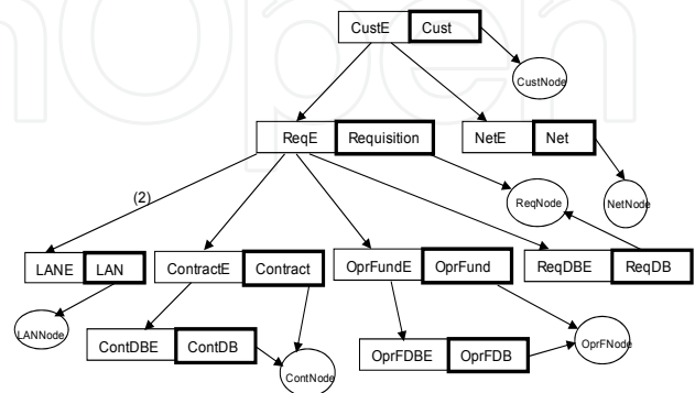
Fig. 8. Centralized LQN model
