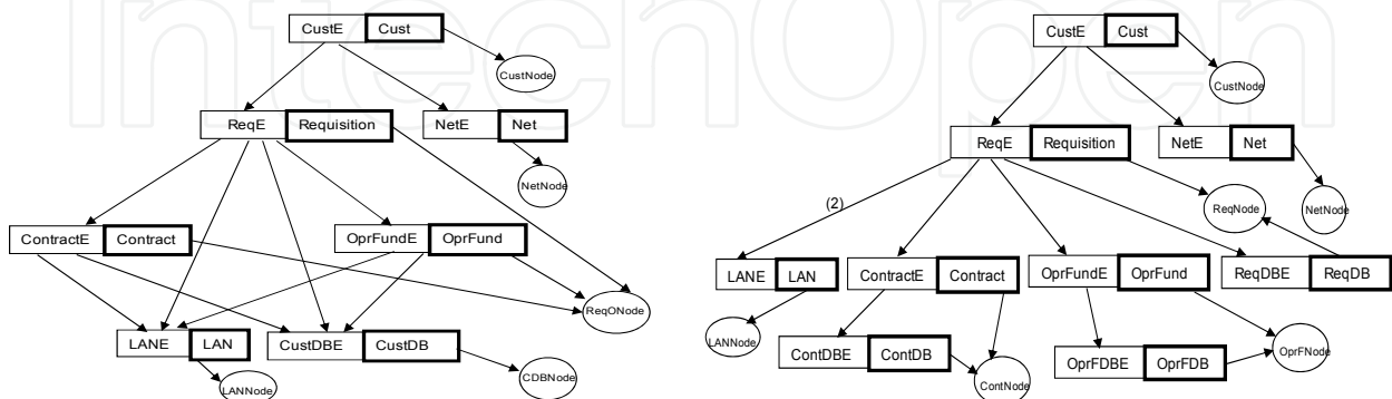
Fig. 8. Centralized LQN model
