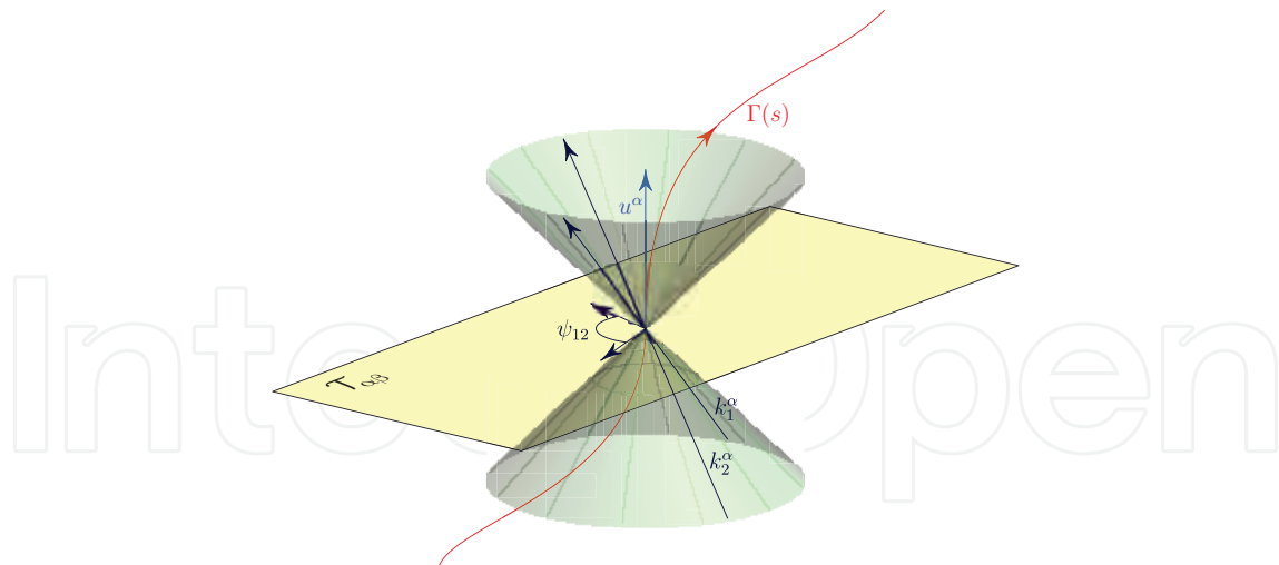
Fig. 4. The formula expressing the arc measured between two directions can be found considering that the relativistic viewing directions k_1^\alpha and k_2^\alpha – i.e. the tangents to the null geodesics connecting the observed objects to the observer and computed at the observation event – have to be projected onto the spatial hypersurface relative to u^\alpha .
