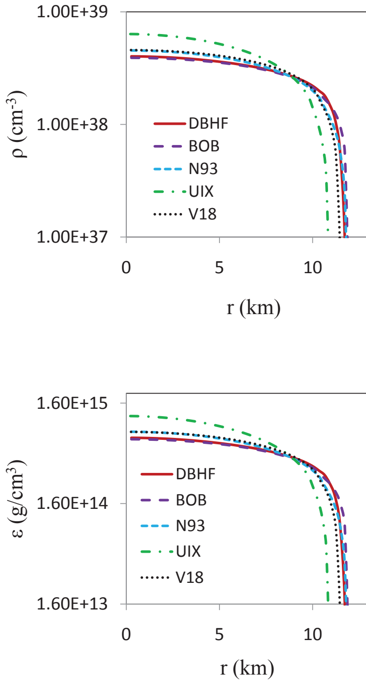
Fig. 10. The baryon density and the mass-energy density profile for a neutron star with a mass of 1.4 solar masses.
