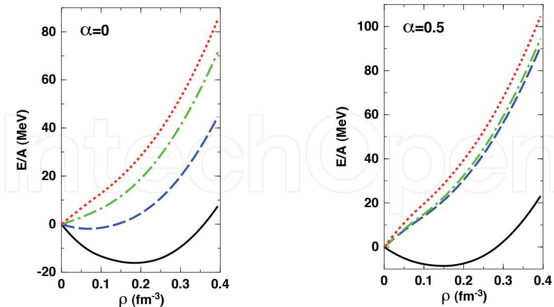
Fig. 20. The energy per particle as a function of density and various degrees of proton and neutron polarizations in symmetric matter (left) and asymmetric matter (right). In both frames, the (blue) dashed line corresponds to totally polarized neutrons and unpolarized protons ( \beta_n=1, \beta_p=0 ); the (green) dash-dotted line is the prediction for the FM state ( \beta_n=1, \beta_p=1 ); the (red) dotted line shows the energy of the AFM state ( \beta_n=1, \beta_p=-1 ). The (black) solid line shows the predictions for unpolarized matter.
