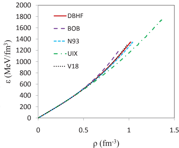
Fig. 13. Energy density vs. baryon number density for the various EoS being addressed in the text. The maximum-mass model is considered in each case.
