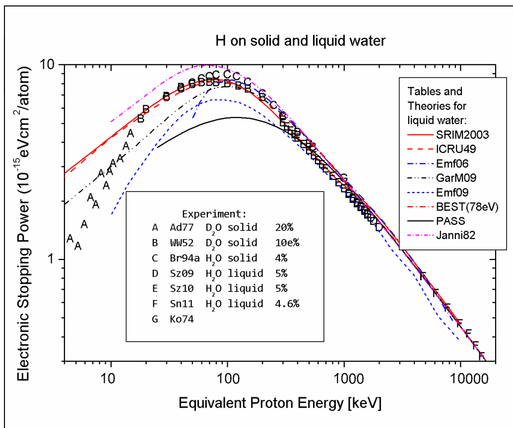
Fig. 7. Electronic stopping power of solid and liquid water for protons, versus energy. The file designations for experiments are explained in Paul (2011a). The table and theory designations are explained in Table 1, except for the following: Emf06 (Emfietzoglou et al, 2006), Emf09 (Emfietzoglou et al., 2009), GarM09 (Garcia-Molina et al., 2009), PASS (Sigmund & Schinner, 2002; Sigmund, 2010)
