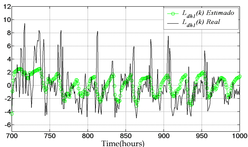
Fig. 22. Comparison between the signal estimated by the linear SISO model and the real signal L_{dh1}(k) .
