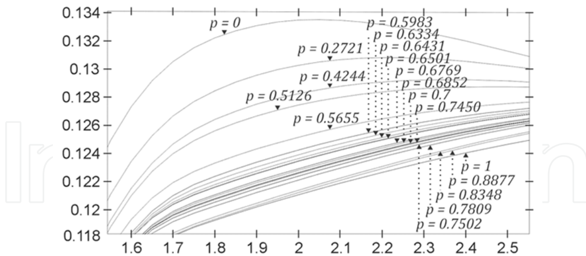
Fig. 11. Transient response for several values of parameter of rule 18
