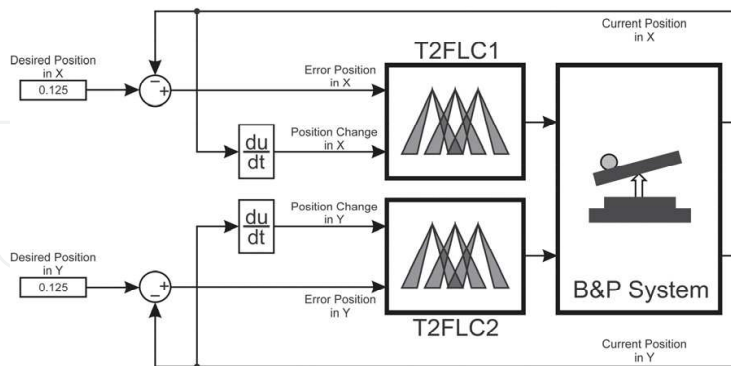
Fig. 5. PT2FLC for B&P System
