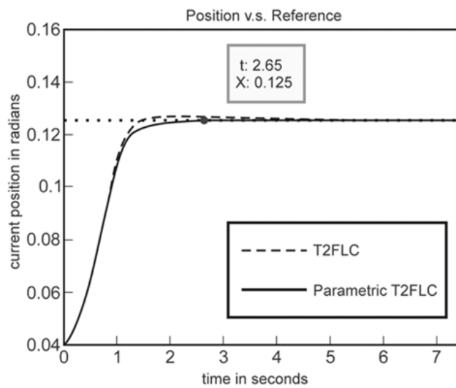
Fig. 13. Final approximation of T2FLC modifying rule parameters
