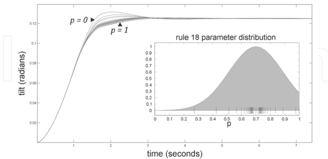
Fig. 10. Rule 18 parameter distribution for 43 experiments
