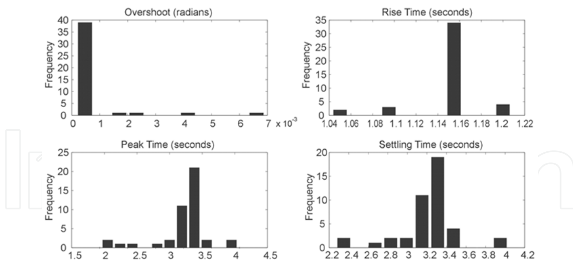
Fig. 12. Histograms for transient measures (overshoot, rise time, peak time and settling time) for rule parameter 18
