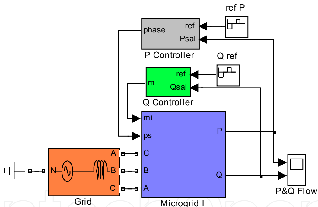
Fig. 25. Block system of three phase grid connected VSC
