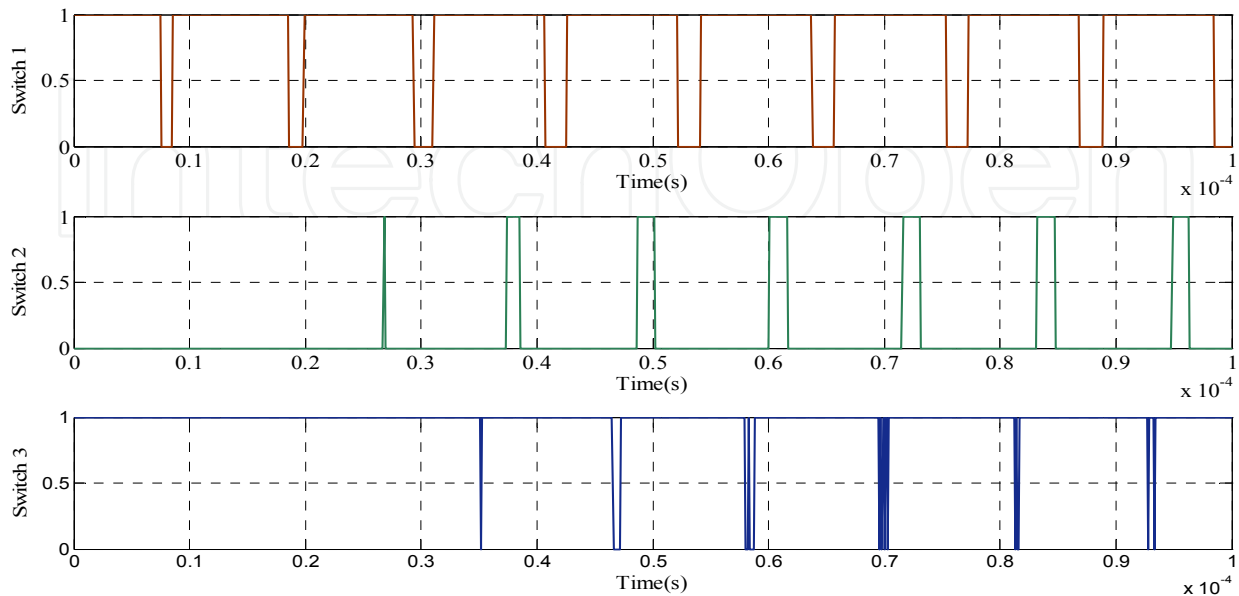
Fig. 9. Self-Switching Pulses
