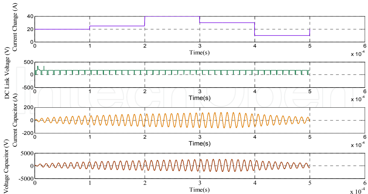
Fig. 11. Current Variability
