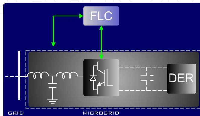
Fig. 23. MG block representation with Fuzzy Logic Controller
