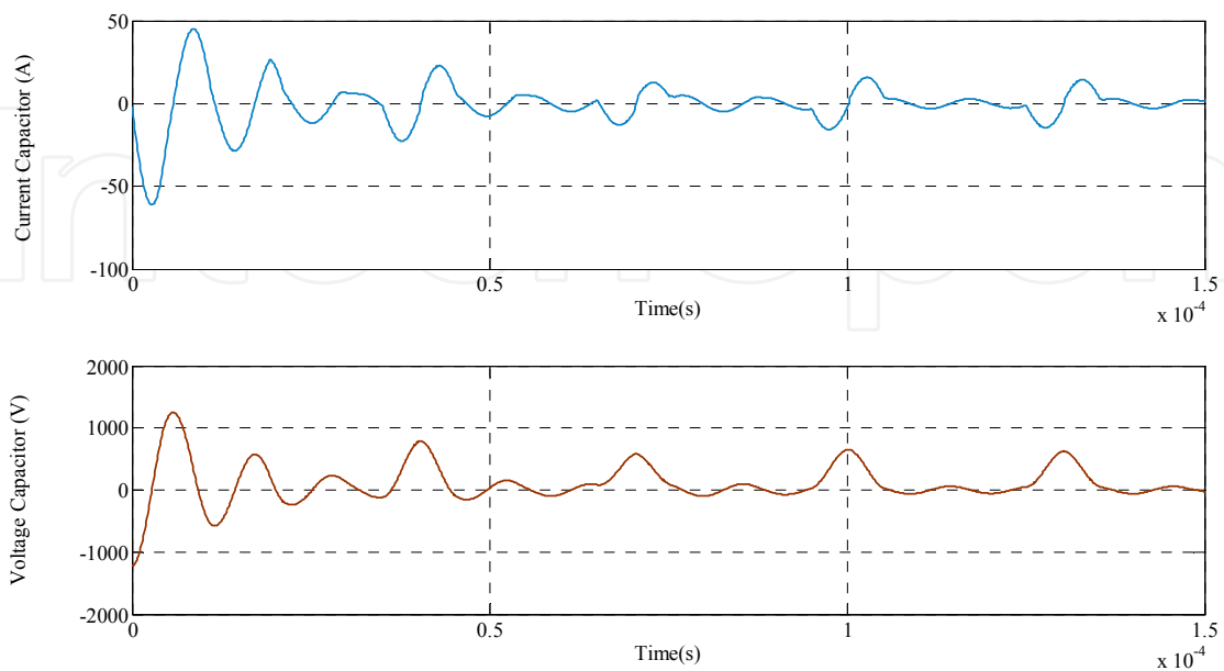
Fig. 4. Current and Voltage Capacitor Waveforms
