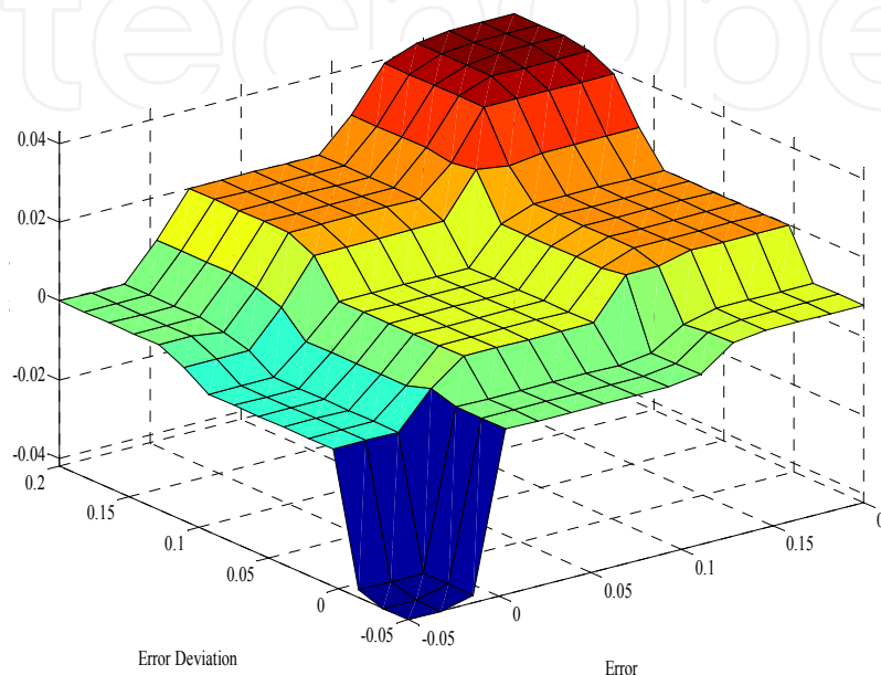
Fig. 18. Control Surface
