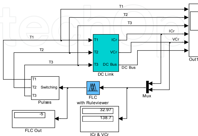
Fig. 8. Closed Loop System
