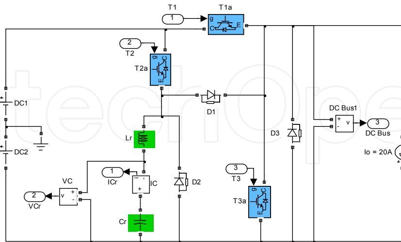
Fig. 3. DC Link Circuit
