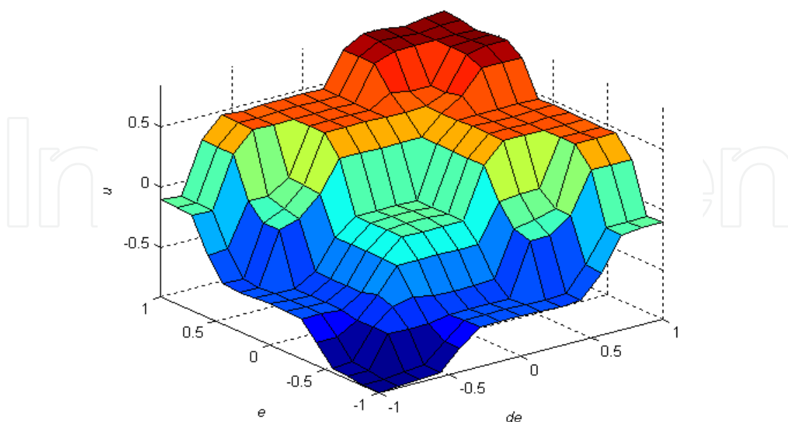
Fig. 12. The output surface of the fuzzy inference system for five fuzzy subsets arranged in asymmetrical shape..
