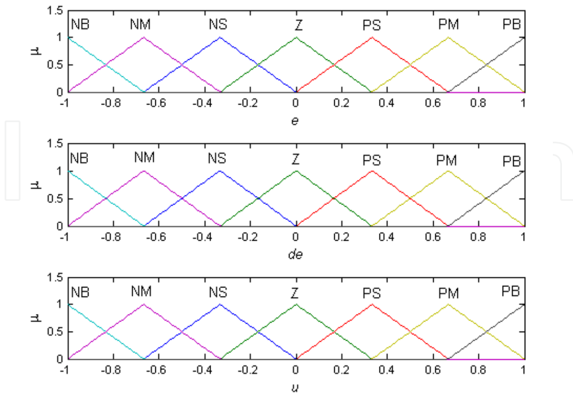
Fig. 7. Membership functions for input e , de and u
