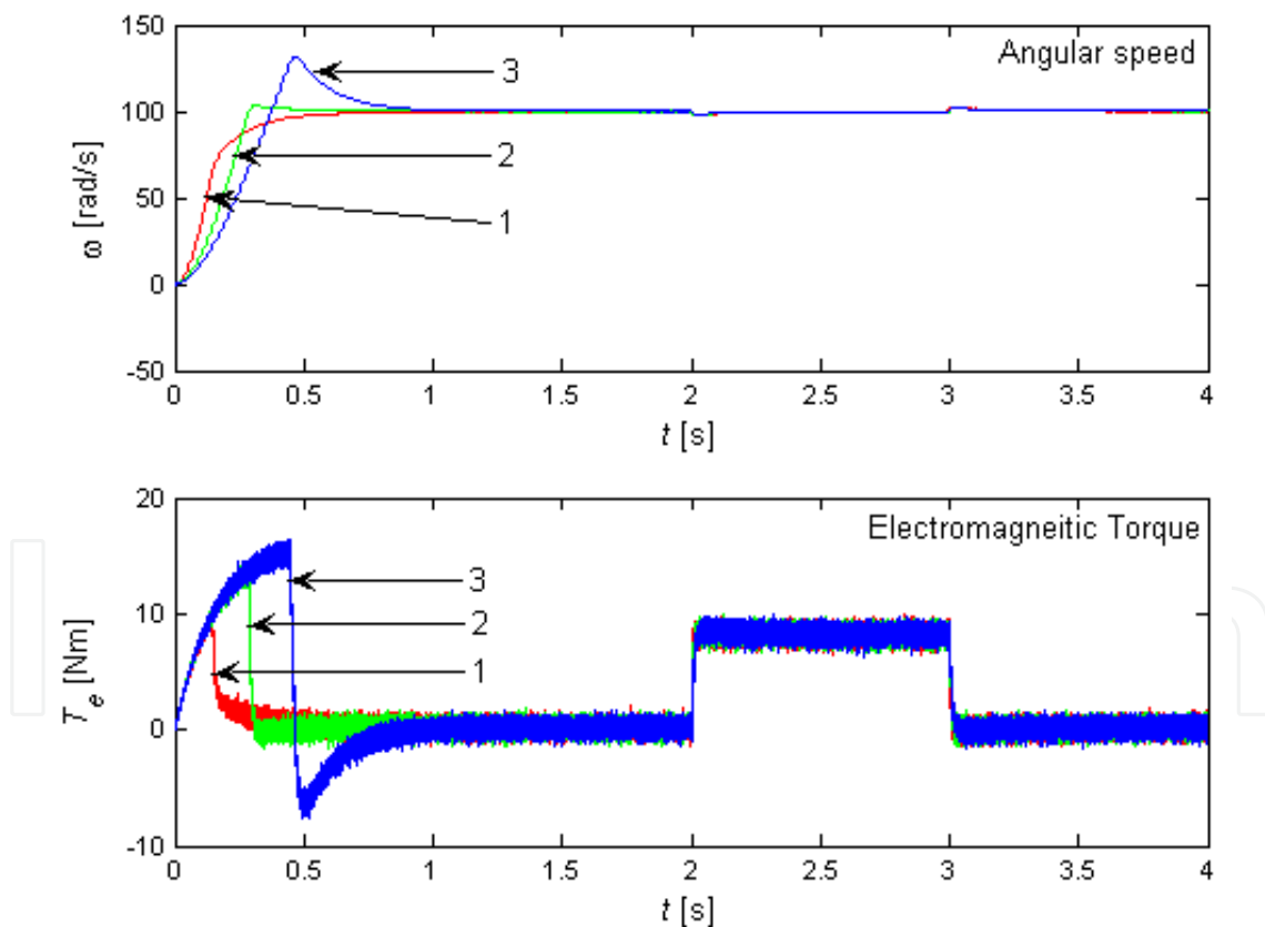
Fig. 23. Test of robustness for different values of the moment of inertia using fuzzy rules of Table 2: 1) -50\% , 2) nominal case, 3) +50\% .
