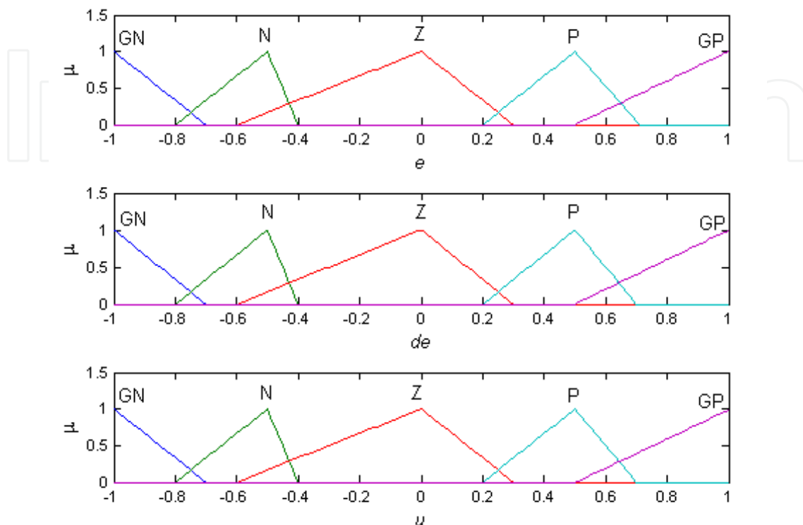
Fig. 11. Membership functions for input e , de et u arranged in asymmetrical shape.
