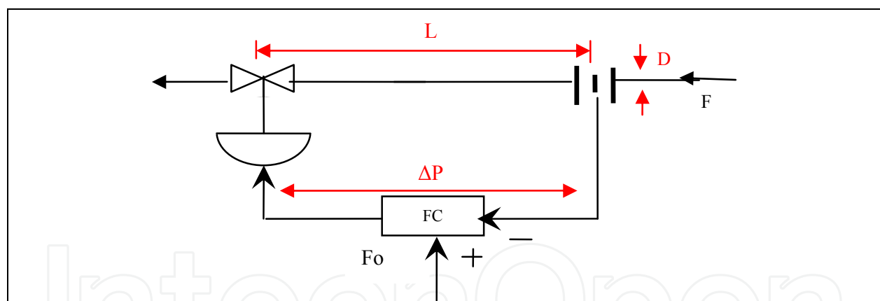
Fig. 3. Flow controller
