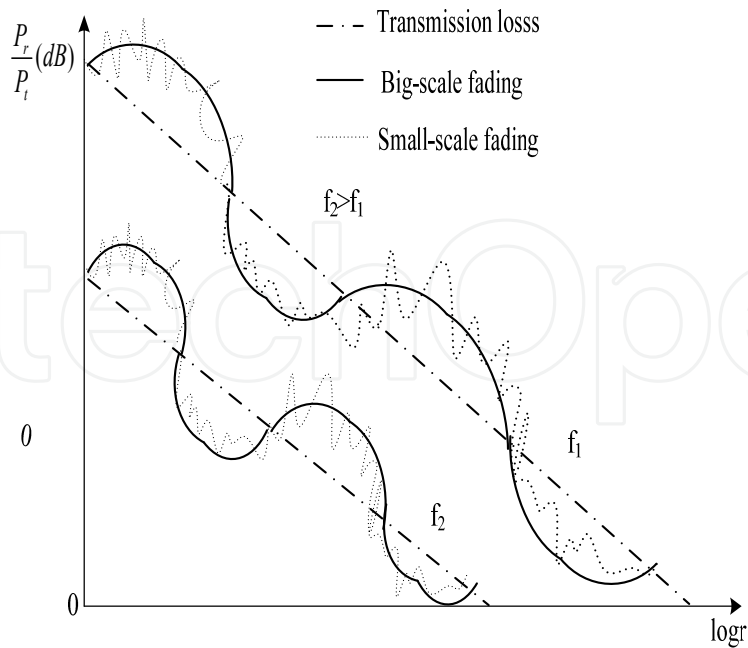
Fig. 1. The relations between range and fading
