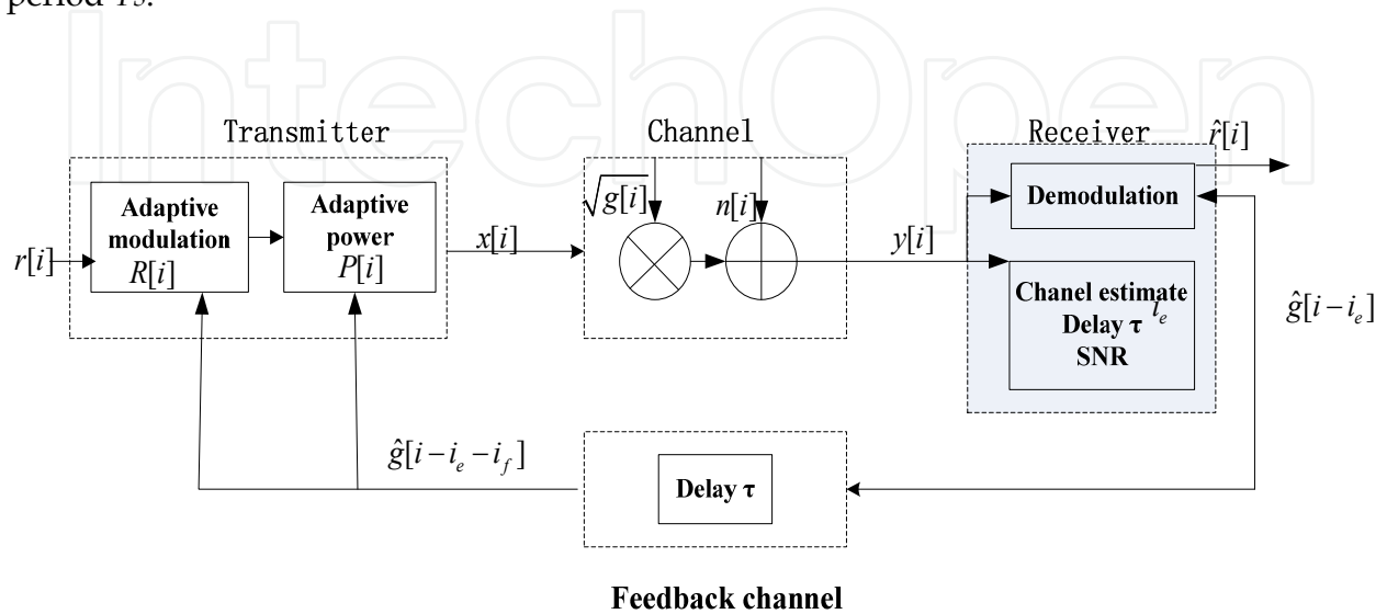
Fig. 4. Block diagram of adaptive system
