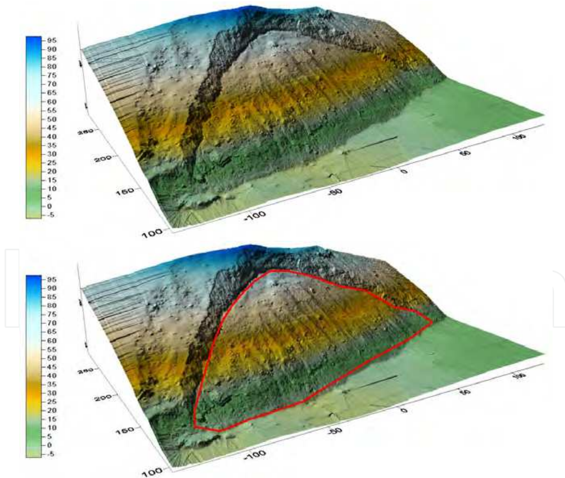
Fig. 7. Triangulated surface of the Locce landslide and selection on the moving/stable areas (red line) for the alignment and movement determination.
