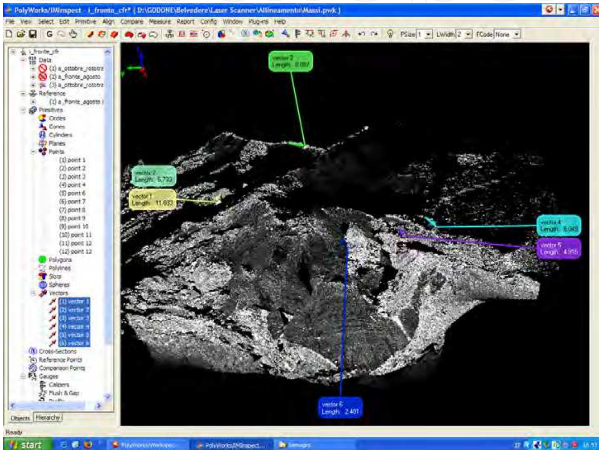
Fig. 15. Vectors plotted on the glacier 3D point cloud
