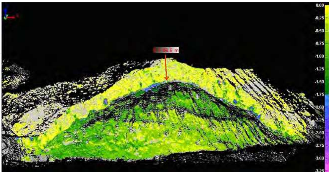
Fig. 13. Measure of the total displacement of the landslide from its edge
