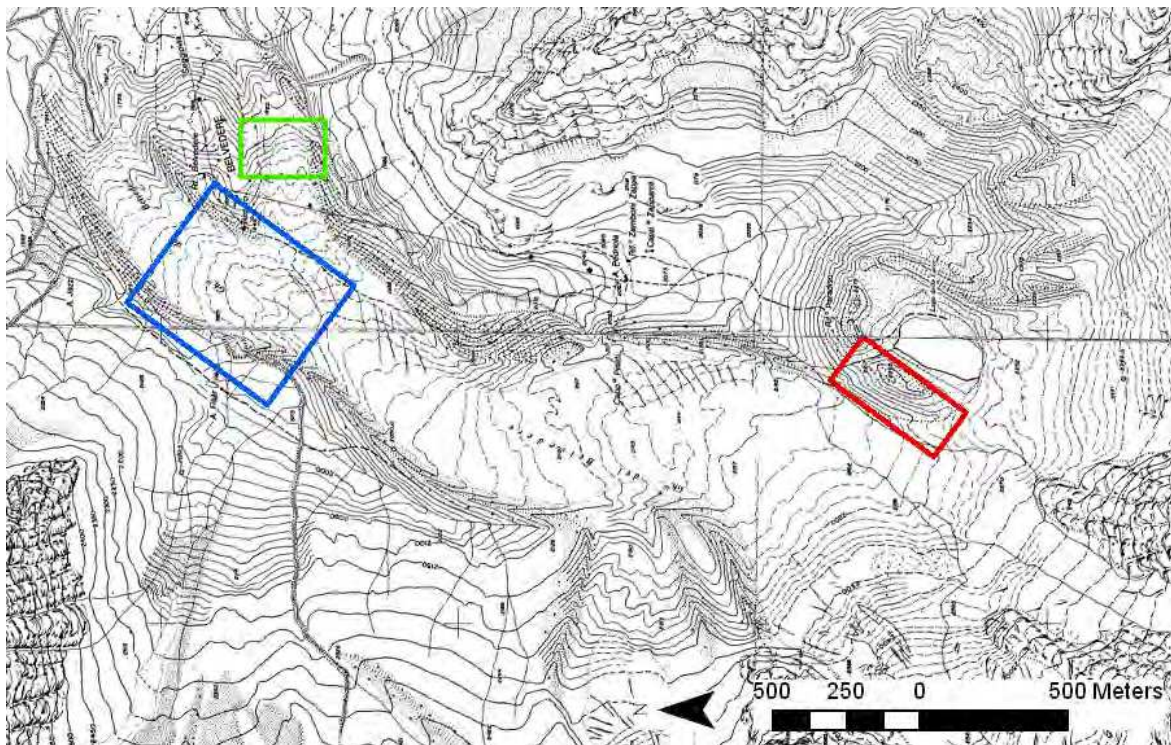
Fig. 3. Terrestrial Laser Scanner survey sites: right snout (green square), Locce landslide (red square) and glacier surface (blues square). Regional Technical Map (original scale 1:10000) in background
