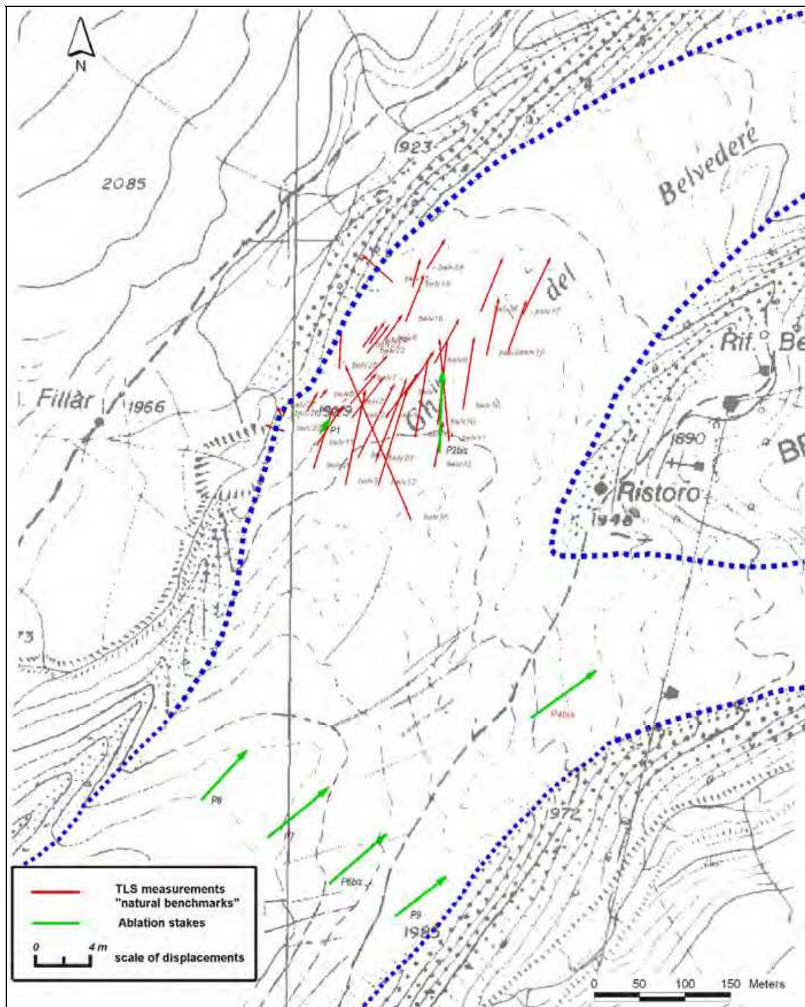
Fig. 18. Displacement measured with TLS on “natural benchmarks” (in red) and from ablation stakes positions (green)
