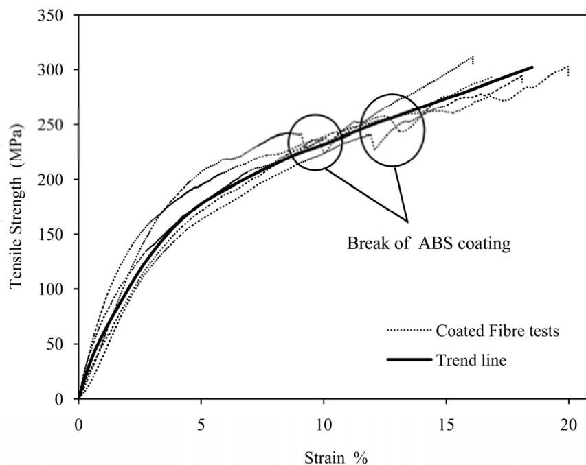
Fig. 6. Stress-strain curve of coated OPEFB fibres on tensile test
