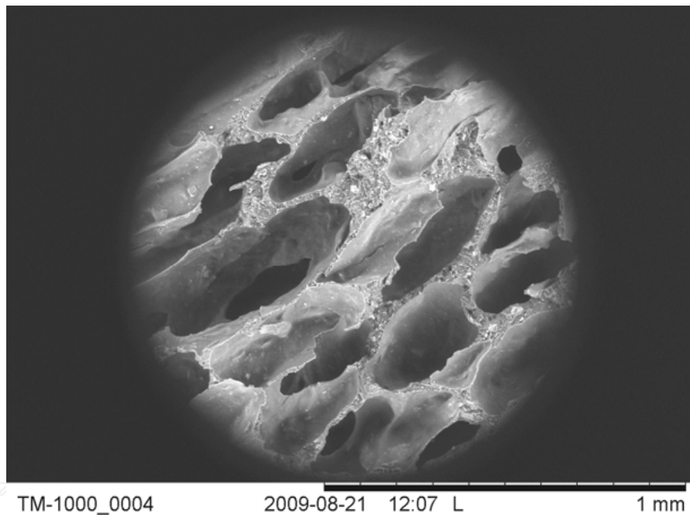
Fig. 10. Structure of polypropylene foam produced with egzothermic CBA
