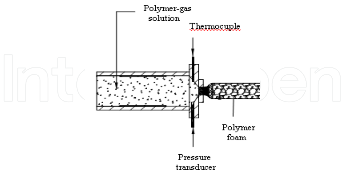
Fig. 13. Polymer foaming extrusion principle
