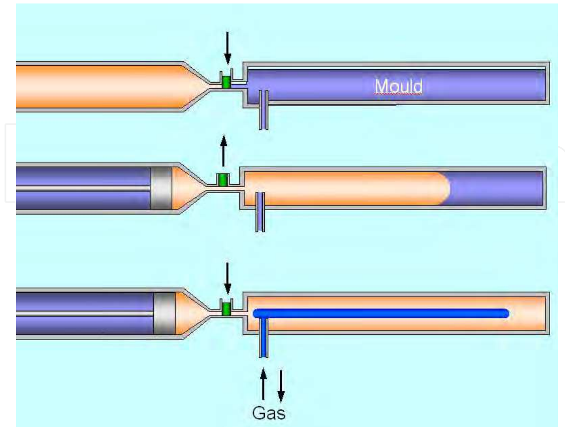
Fig. 6. Principle of gas-assisted injection molding (acc. to www.cinpres.net )
