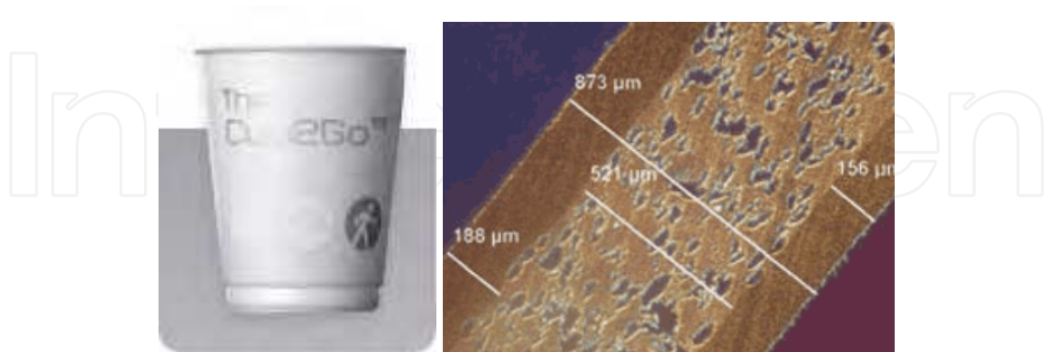
Fig. 12. Foamed polystyrene cup and its wall structure (acc. to www.adeka-palmarole.com )
