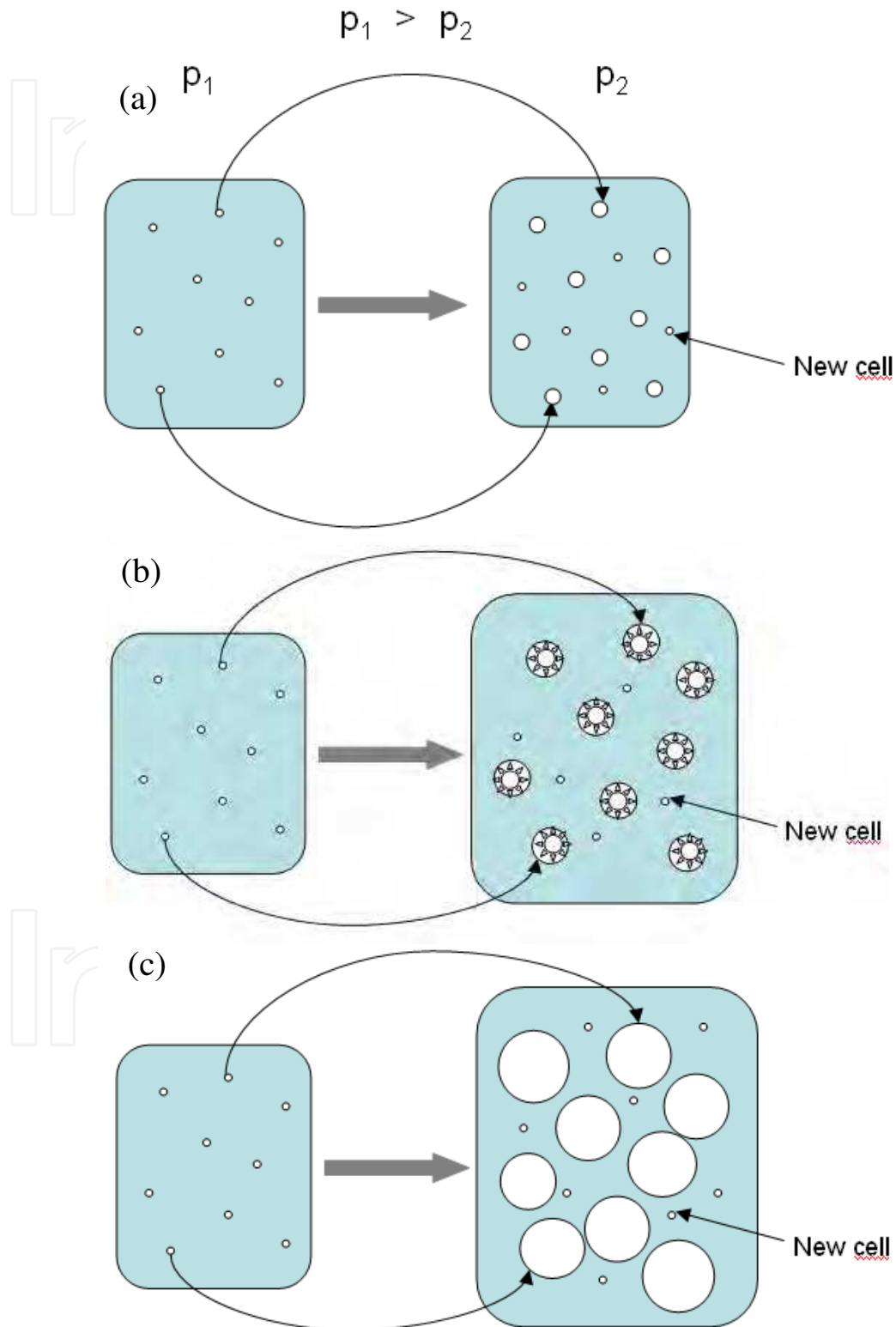
Fig. 16. Schematic representation of extrusion foaming stages
