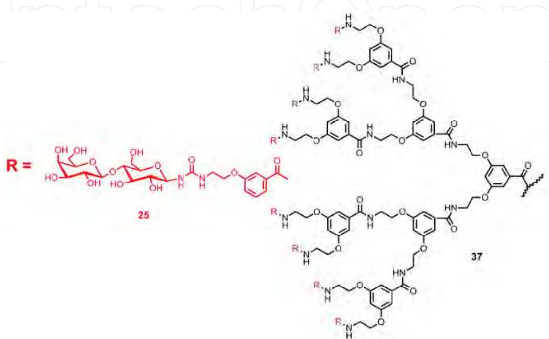
Fig. 17. A scheme of Pieters' multivalent inhibitor based on dendridic structure.
