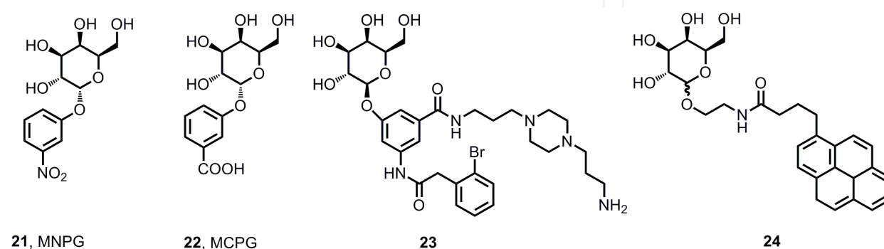
Fig. 8. Some examples from MNPG (MCPG) library.
