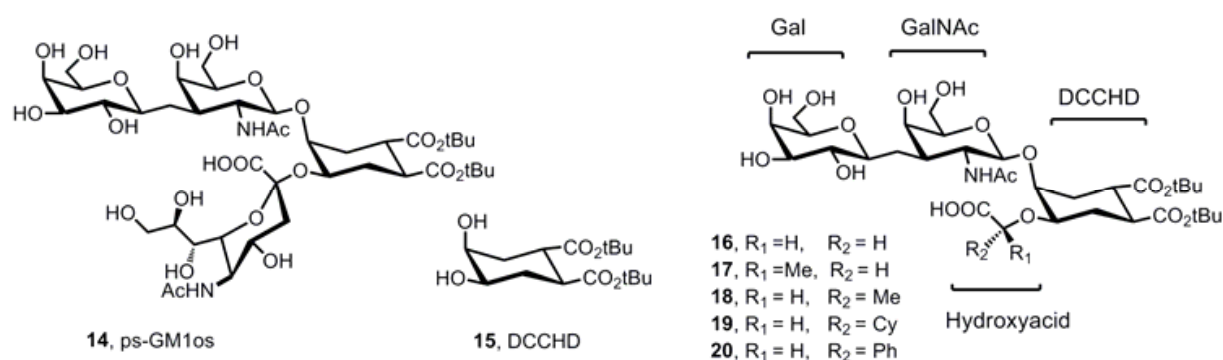
Fig. 6. Structures of Bernardi's GM1 mimics.
