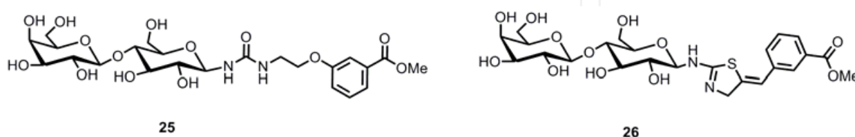
Fig. 10. Pieters' lactose derived ligands.
