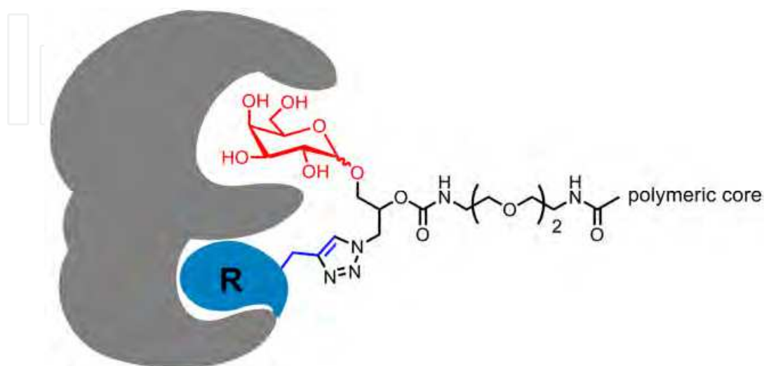
Fig. 19. Scheme for general design of multivalent Tran-Kitov's bidentate inhibitors.
