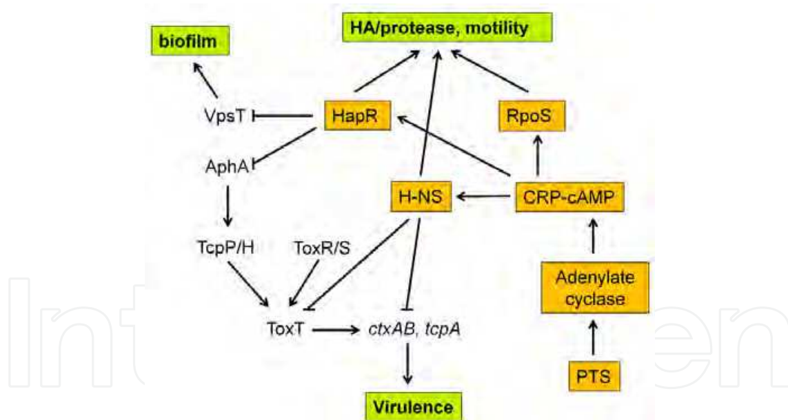
Fig. 16. Multilevel regulation of V. cholerae behavior by CRP.
