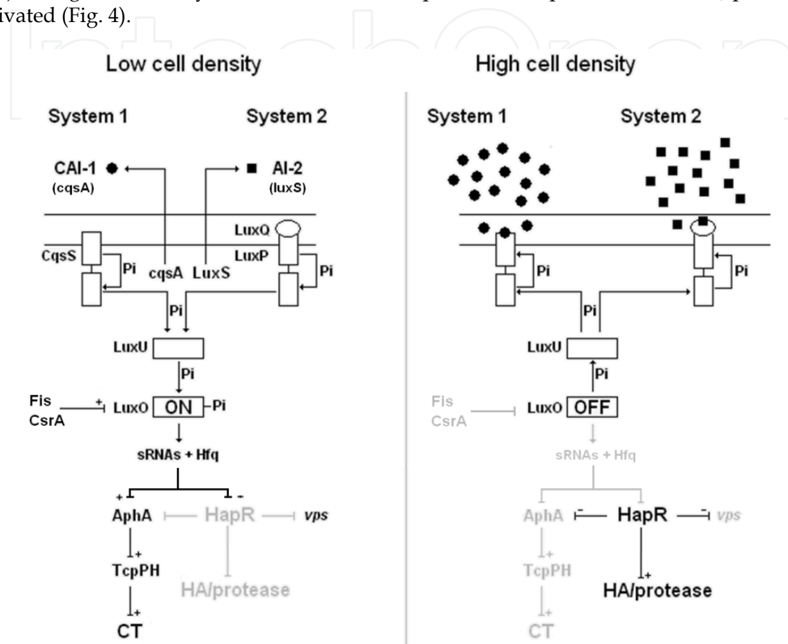
Fig. 4. Quorum sensing in Vibrio cholerae
