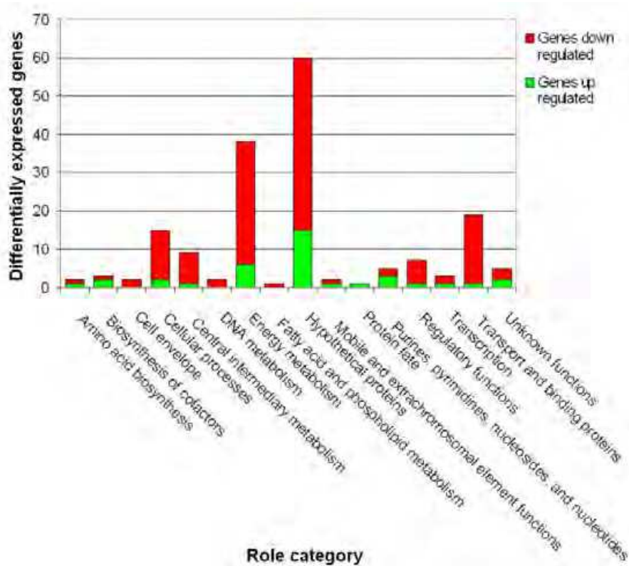
Fig. 6. Global regulation by the cAMP receptor protein.
