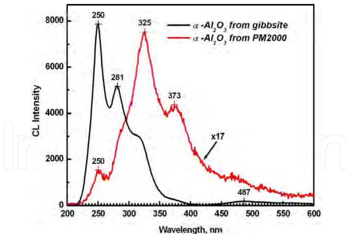
Fig. 9. CL spectra of \alpha - Al_2O_3 , formed by calcination of gibbsite powder at 1573 K for 24 h (black line) and by oxidation of PM2000 at 1223K for 72h (red line), obtained in the region of 200 to 600 nm at room temperature.
