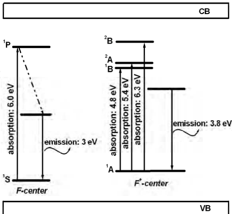
Fig. 10. Schematic energy level diagram for absorption and emission of F- and F + -centres in \alpha -Al 2 O 3 crystal.
