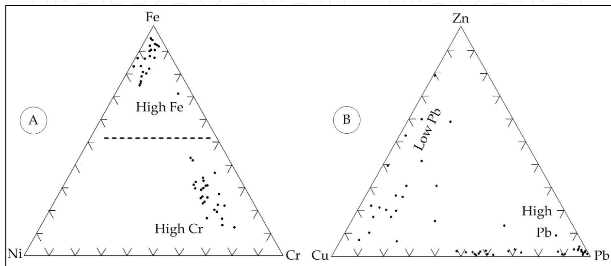
Fig. 10. Mutual relationships among A) Ni-Fe-Cr and B) Cu-Zn-Pb showing two populations of soil samples in the study area.
