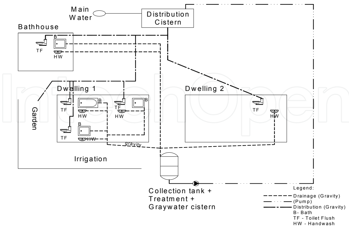
Fig. 5. Greywater system.
