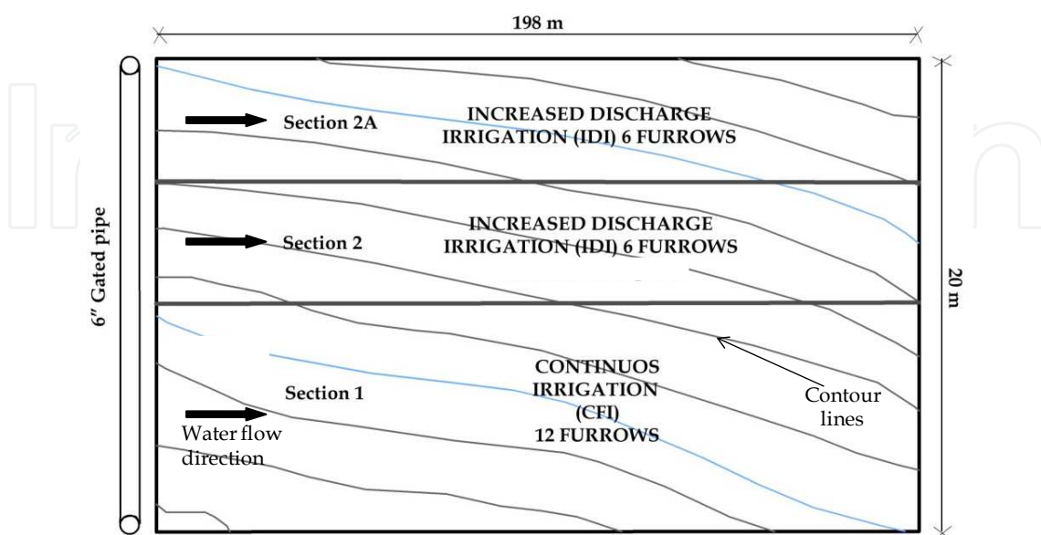
Fig. 4. Topographical diagram for experimental plot
