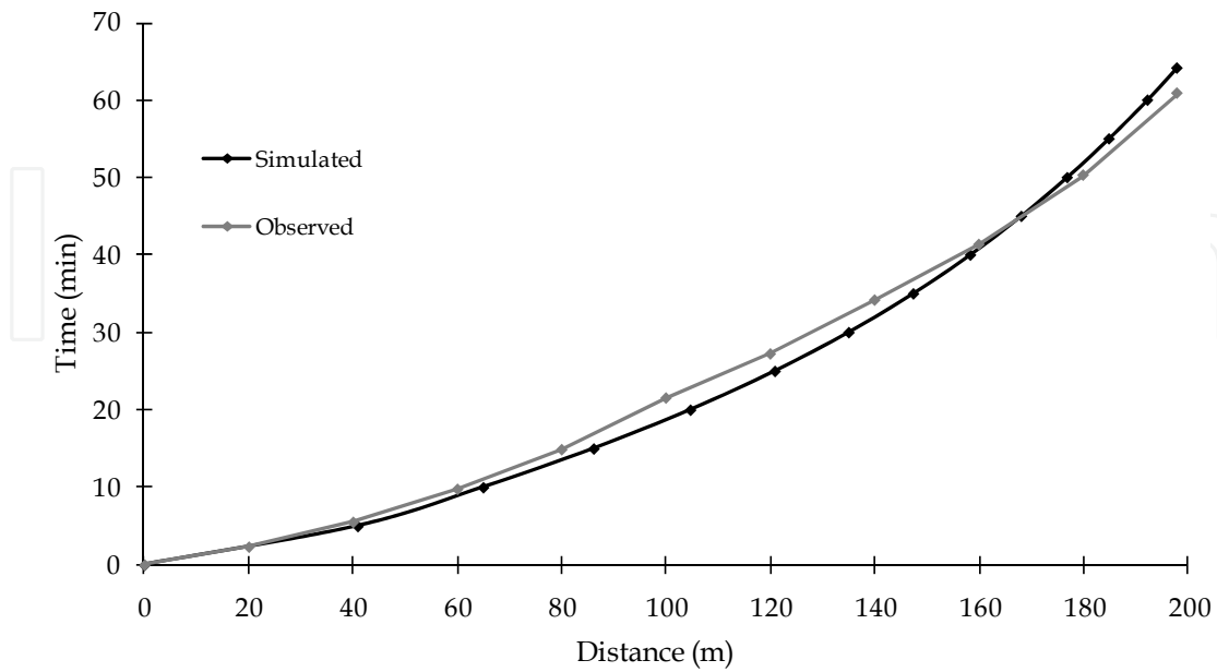
Fig. 6. Water advance curves. Pre-sowing irrigation for CFI (2004)
