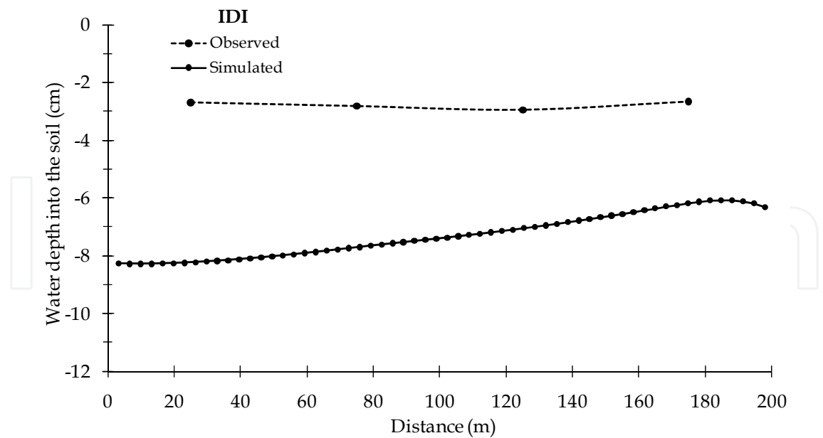
Fig. 12. Infiltration table along furrow for IDI. Observed values were monitored in 2004
