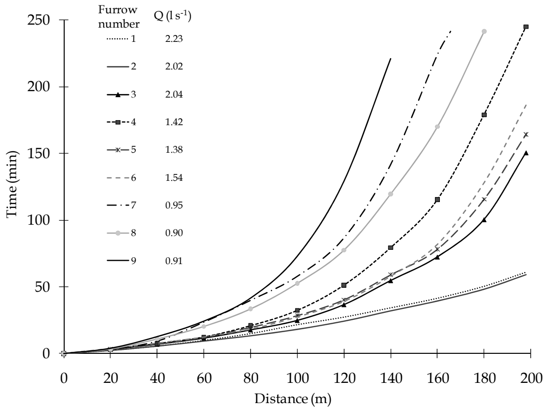
Fig. 5. Family water advance curves
