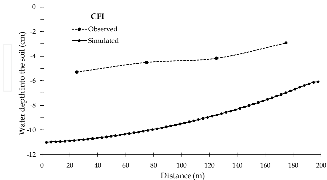
Fig. 11. Infiltration table along furrow for CFI. Observed values were monitored in 2004
