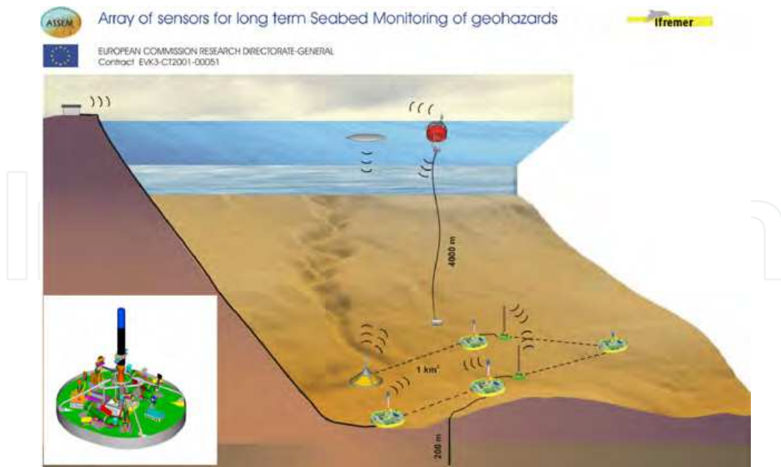
Fig. 5. An ASSEM node and a sketch of multi ASSEM node system ©Ifremer
