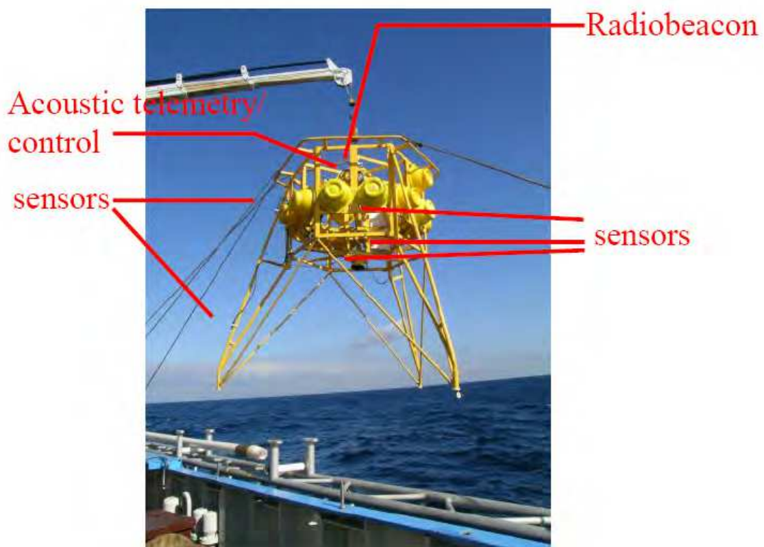
Fig. 1. BOBO lander in previous version (source: http://mars-srv.oceanlab.iu-bremen.de/infra_observ_bobo.html )
