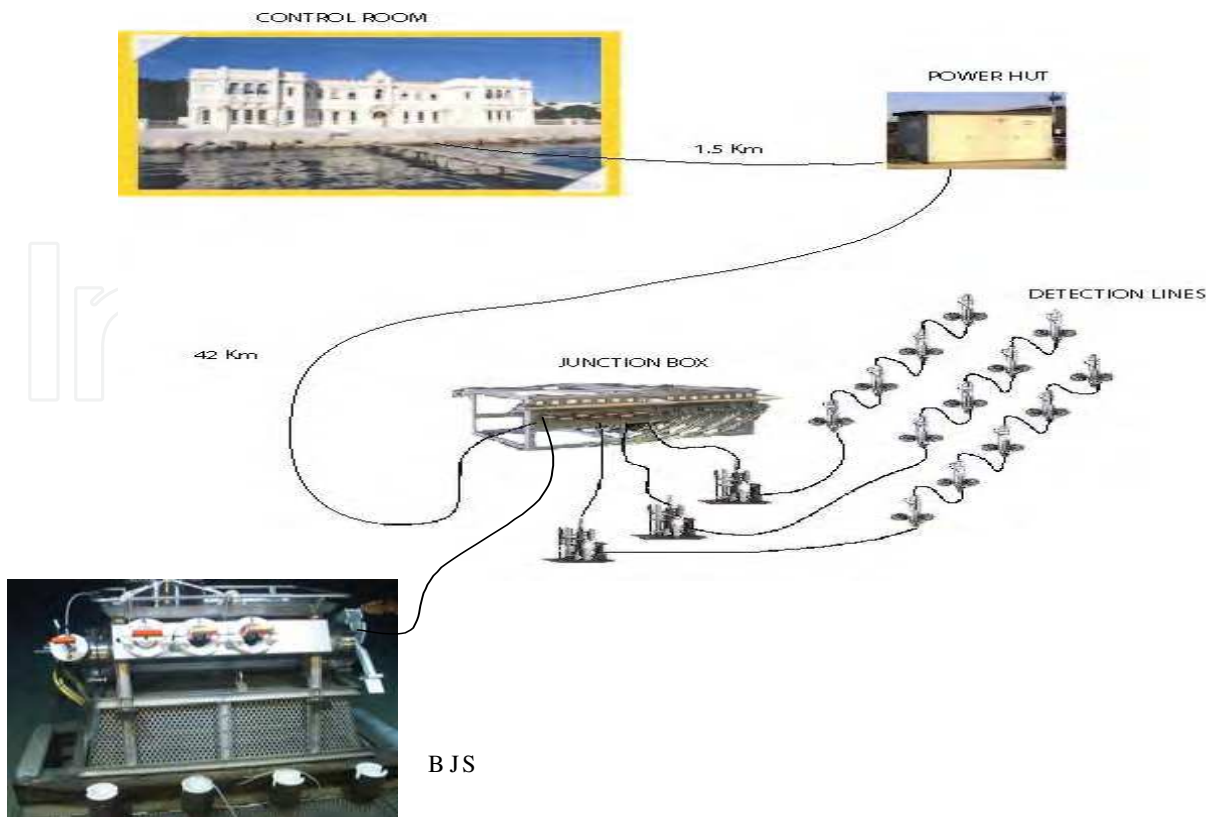
Fig. 9. Scheme of the ANTARES cable network (source: Ifremer and CNRS/CPPM)
