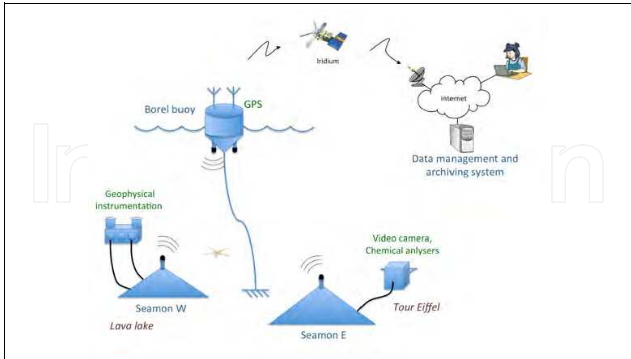
Fig. 14. MOMAR observatory concept
