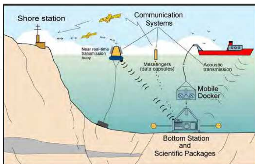
Fig. 4. GEOSTAR bottom station (from Favali and Beranzoli, 2009)
