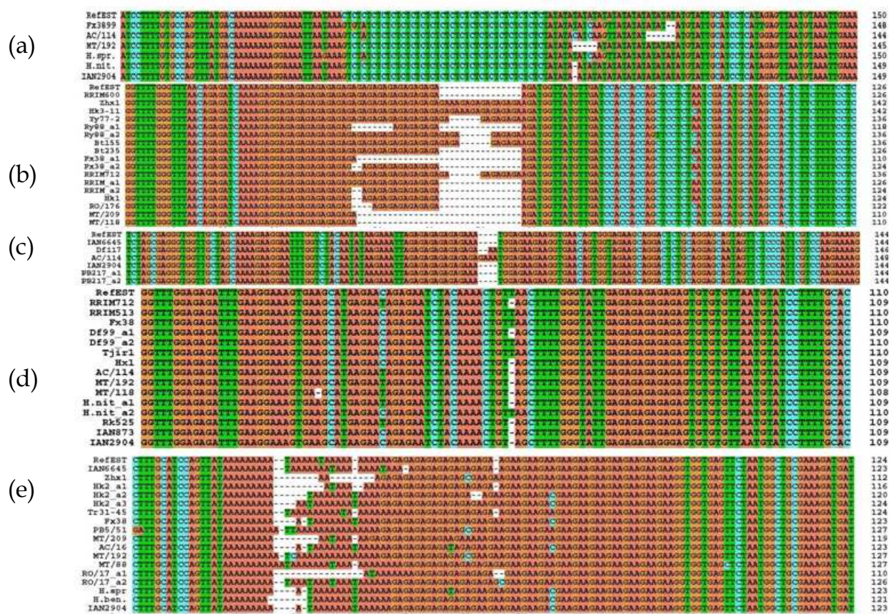
Fig. 2. Sequences obtained using 5 EST-SSRs markers amplifying across H. brasiliensis , wild H. brasiliensis and interspecies. (a), (b), (c), (d) and (e) (from the top down) represent the markers HBE008, HBE063, HBE164, HBE187 and HBE199, respectively; RefESTs in (a), (b), (c), (d), (e) represent the accession numbers: EC609578.1, EC607362.1, EC603146.1, EC601817.1 and EC600890.1 in NCBI database, respectively. The suffix 'a1', 'a2' and 'a3' represent the allele numbers. AC/114, MT/192, RO/176, MT/209, MT/118, RO/17, MT/88, AC/16, Zhx1, Ry88, Bt155, Hk3-11, Hk1, Bt235, Yy77-2, Fx38, Df117, Df99, Hx1, Rk525, Hk2, Tr31-45, RRIM, H.spr., H.nit., H.ben., represent AC/T/15/114, MT/IT/1634/192, RO/C/923/176, MT/IT/1634/209, MT/IT/1430/118, RO/CM/1163/17, MT/C/1017/88, AC/AB/1554/16, Zhenxuan1, Reyan88-13, Baoting155, Hekou3-11, Haiken1, Baoting235, Yunyan77-2, Fx3899, Dafeng117, Dafeng99, Hongxing1, Reken525, Haiken2, Tianren31-45, RRIM513, H. Spruceana , H. Nitida , Hevea. Benthamiana , respectively.
