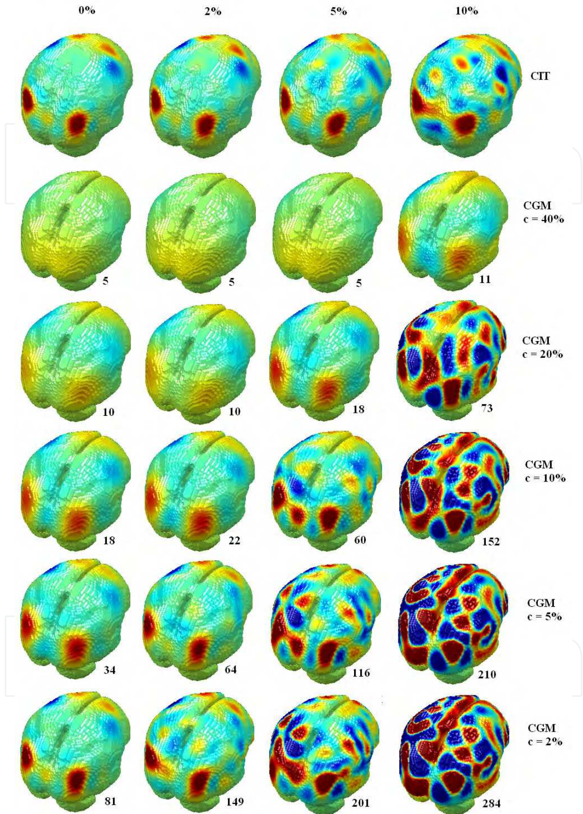
Fig. 5. CIT and CGM 107 electrodes (equation 14)
