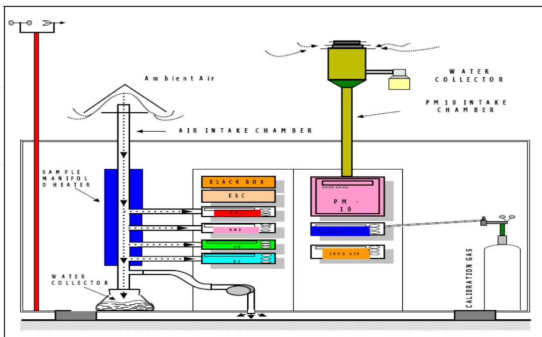
Fig. 3. Schematic Diagram of CAQM (Source: DOE, 2008).
