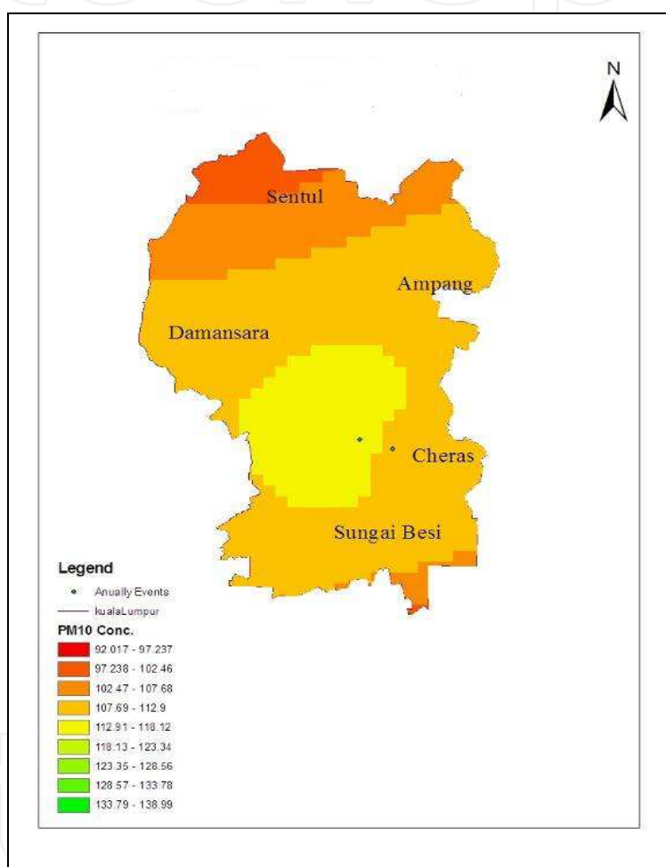
Fig. 12. Maximum PM 10 Concentration at Kuala Lumpur from 2004-2008.
