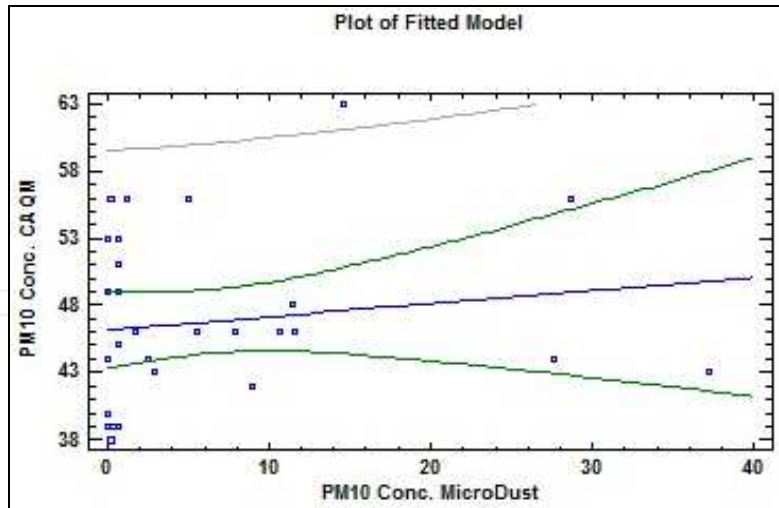
Fig. 17. Regression between CAQM data and Casella Mircodust Pro data.
