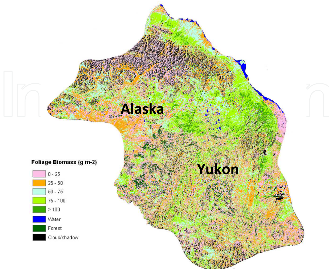
Fig. 10. Foliage biomass distribution over the Porcupine caribou habitat circa 2000. The 3-d effect was generated using the DEM data. Areas covered by water, forest, and cloud were blocked out.
