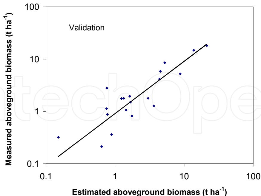
Fig. 7. A 1:1 comparison between estimated and measured aboveground biomass values for the validation sites along the Dempster Highway transect measured during the summer of 2006 and in the Ivvavik National Park during the summer of 2008. For clarity over the low biomass range, the results are shown on the log-log scale.
