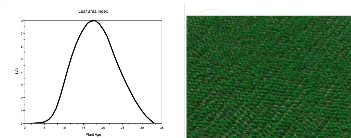
Fig. 3. Synthetic result from GreenLab model. (a) simulated LAI dynamics of virtual maize from GreenLab model; (b) top view of a virtual maize field;
